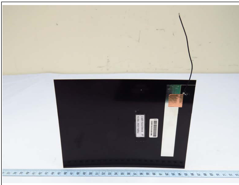
Antenna No. 5
