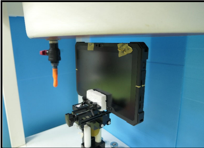
Top Side of EUT Tested at 15 mm
