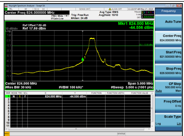
16QAM Low channel-1 RB offset 0
