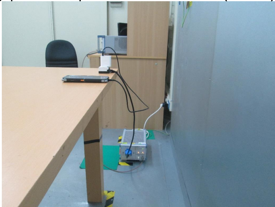
Photograph 50: Test Setup for Mains Conducted Emissions (Back View)
