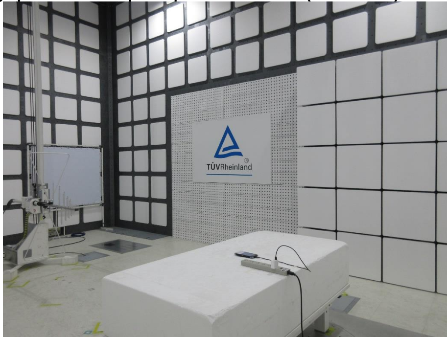
Photograph 47: Test Setup for Spurious Emissions (Back View 2)
