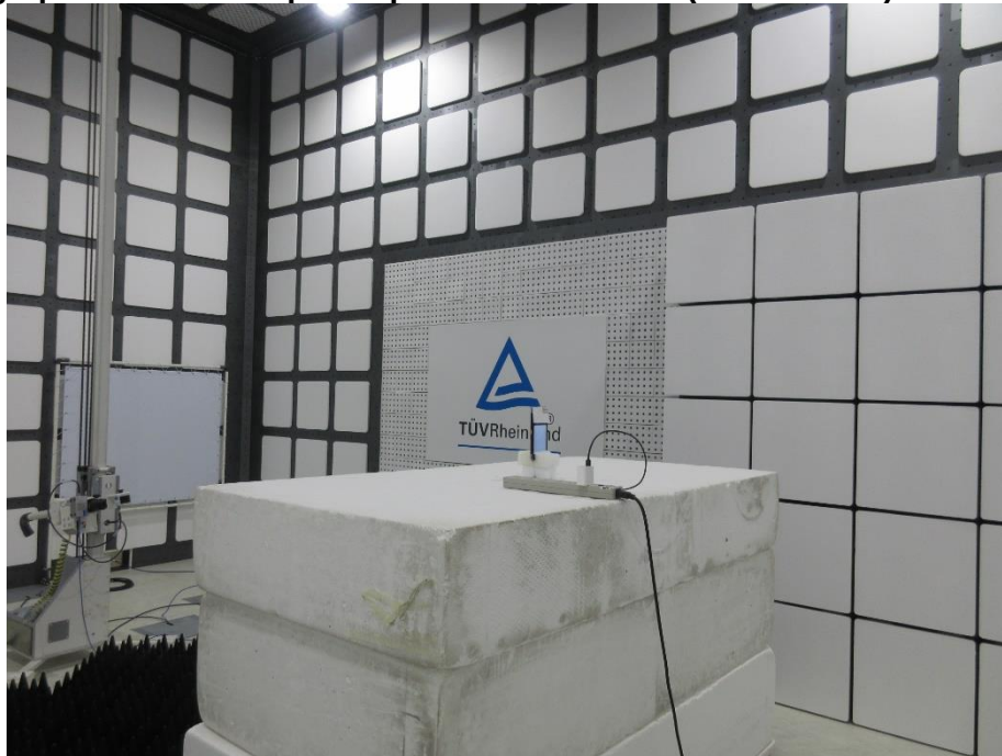
Photograph 43: Test Setup for Spurious Emissions (Back View 3)
