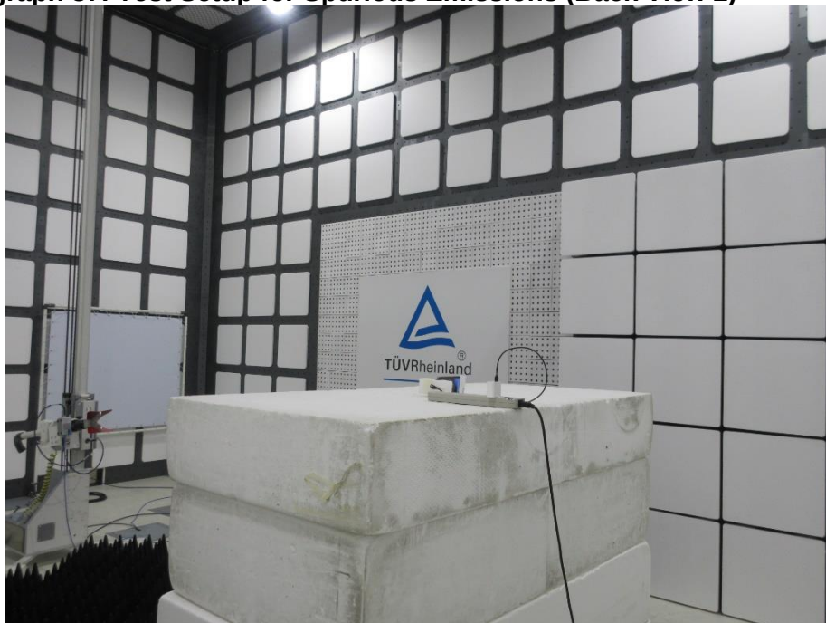
Photograph 37: Test Setup for Spurious Emissions (Back View 2)
