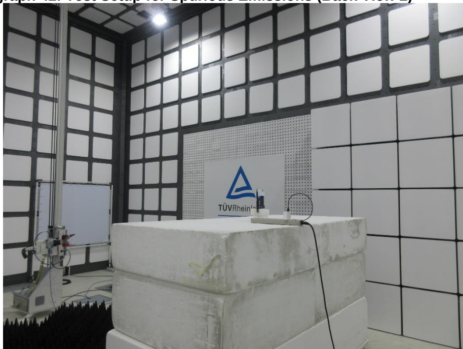
Photograph 42: Test Setup for Spurious Emissions (Back View 2)
