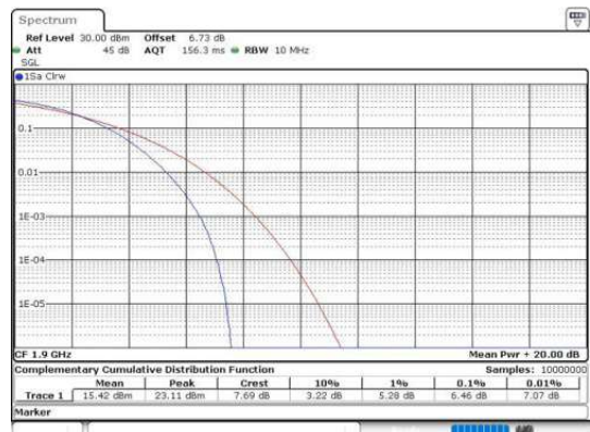
Band2-20MHz-64QAM-19100-100RB#0-PASS
