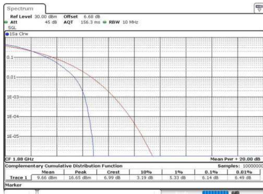
Band2-20MHz-64QAM-19100-1RB#0-PASS
