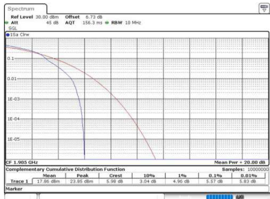
Band2-10MHz-16QAM-19150-50RB#0-PASS
