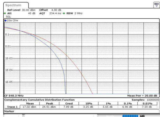
Band5-1.4MHz-64QAM-20643-6RB#0-PASS
