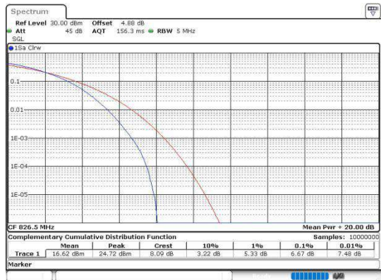
Band5-5MHz-64QAM-20525-25RB#0-PASS
