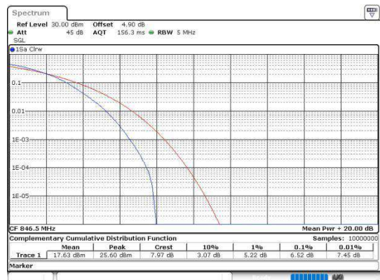
Band5-5MHz-16QAM-20625-25RB#0-PASS
