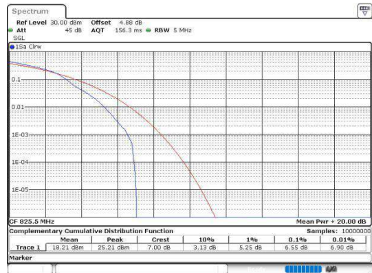
Band5-3MHz-16QAM-20415-15RB#0-PASS
