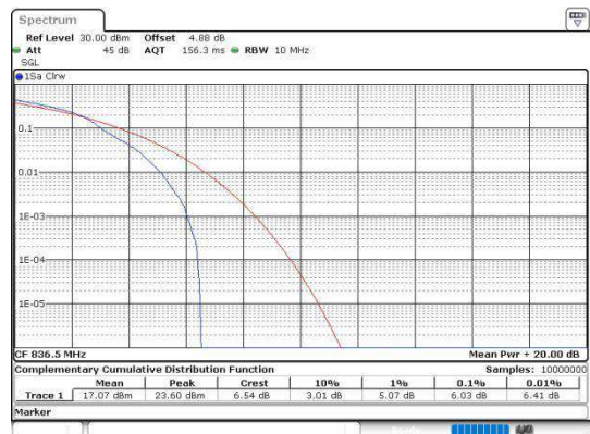
Band5-10MHz-16QAM-20525-1RB#0-PASS
