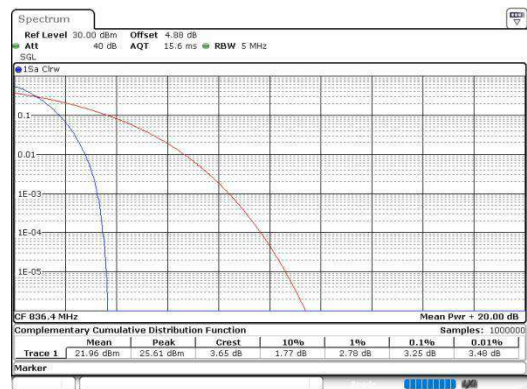
Band5-4182-PASS
