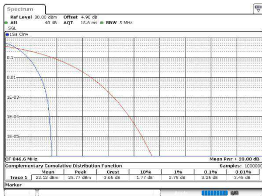
Band5-4233-PASS
