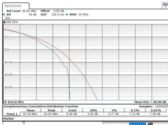
Band5-10MHz-64QAM-20600-1RB#0-PASS
