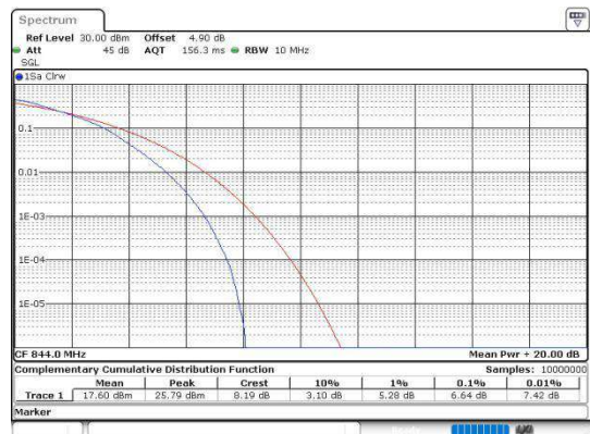
Band5-10MHz-16QAM-20600-50RB#0-PASS
