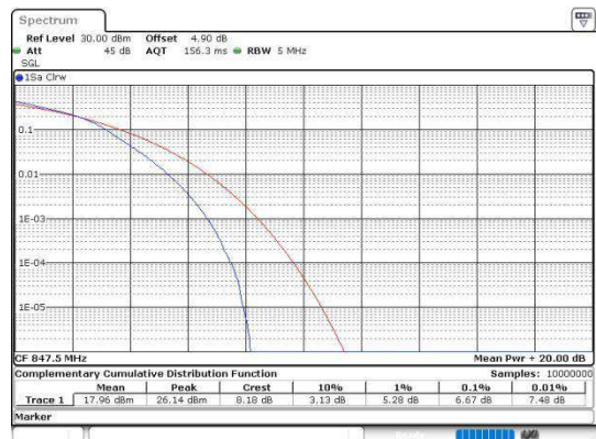
Band5-3MHz-16QAM-20635-15RB#0-PASS
