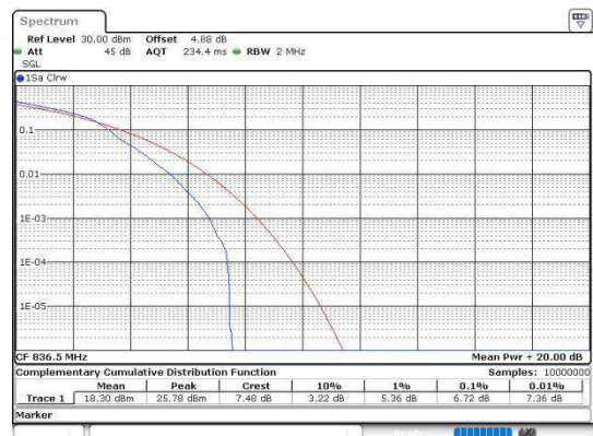
Band5-1.4MHz-16QAM-20525-1RB#0-PASS
