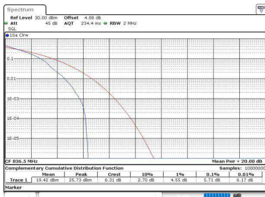
Band5-1.4MHz-QPSK-20525-1RB#0-PASS
