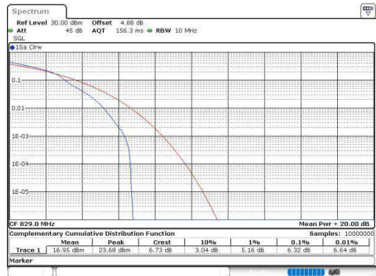
Band5-10MHz-16QAM-20450-50RB#0-PASS
