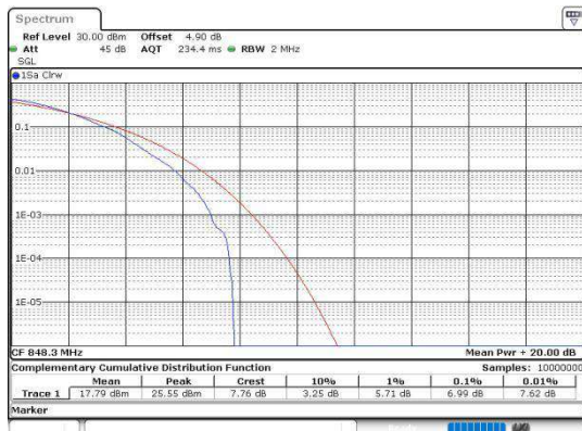
Band5-1.4MHz-64QAM-20643-1RB#0-PASS
