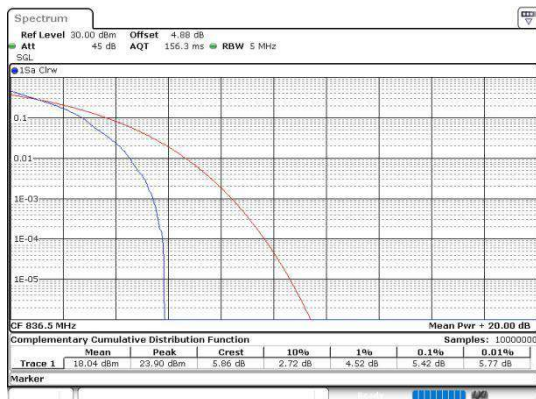
Band5-5MHz-QPSK-20525-1RB#0-PASS
