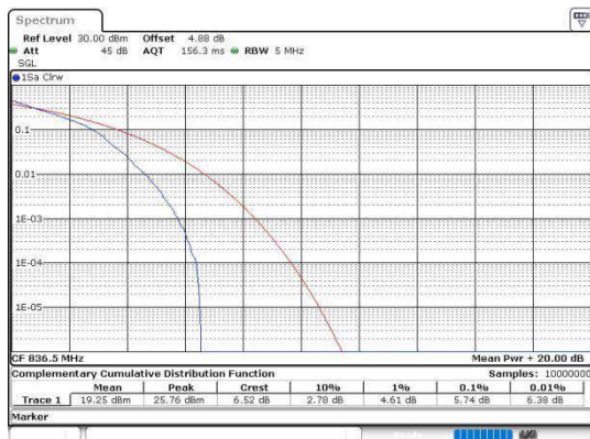
Band5-3MHz-QPSK-20525-1RB#0-PASS
