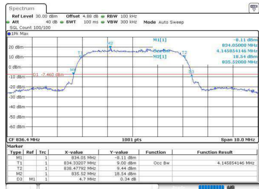
Band5-4182-PASS
