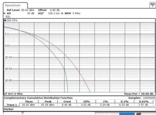
Band5-3MHz-64QAM-20635-15RB#0-PASS
