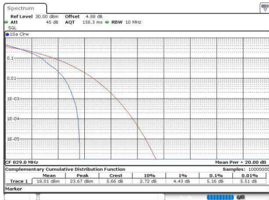
Band5-10MHz-QPSK-20450-50RB#0-PASS
