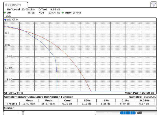
Band5-1.4MHz-16QAM-20407-6RB#0-PASS
