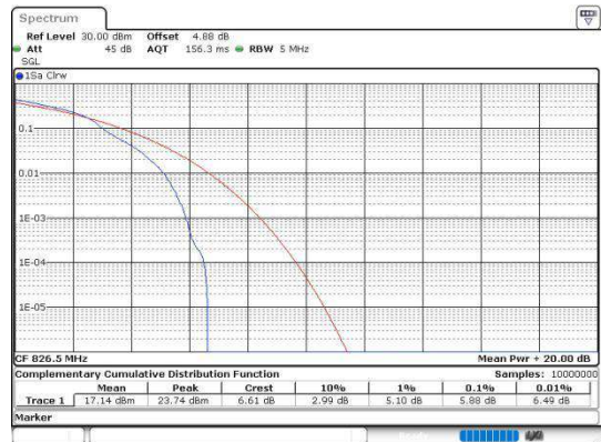
Band5-5MHz-16QAM-20425-25RB#0-PASS
