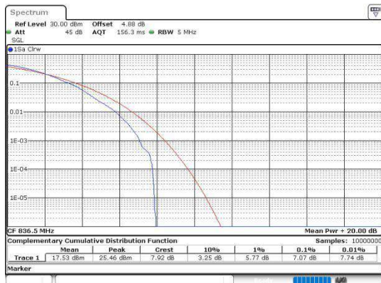
Band5-3MHz-64QAM-20635-1RB#0-PASS
