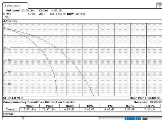
Band5-10MHz-QPSK-20600-50RB#0-PASS
