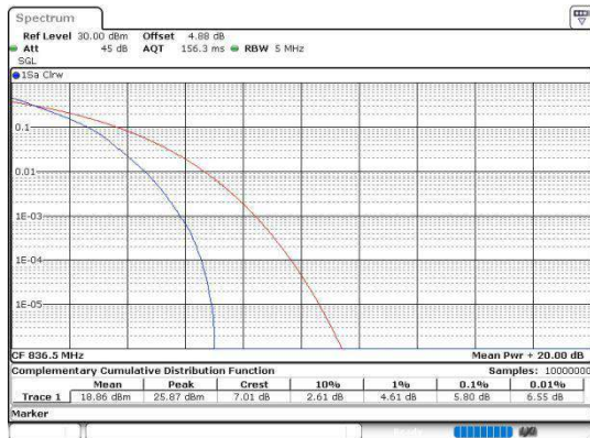
Band5-3MHz-QPSK-20635-1RB#0-PASS
