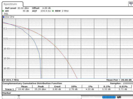
Band5-1.4MHz-QPSK-20407-6RB#0-PASS
