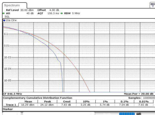
Band5-5MHz-64QAM-20625-1RB#0-PASS
