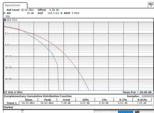
Band5-3MHz-16QAM-20525-1RB#0-PASS
