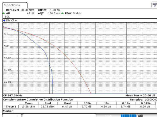
Band5-3MHz-QPSK-20635-15RB#0-PASS
