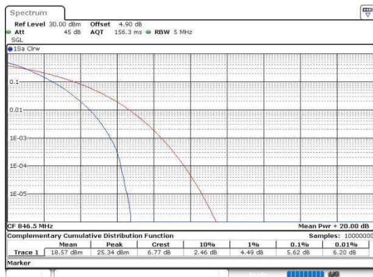
Band5-5MHz-QPSK-20625-25RB#0-PASS
