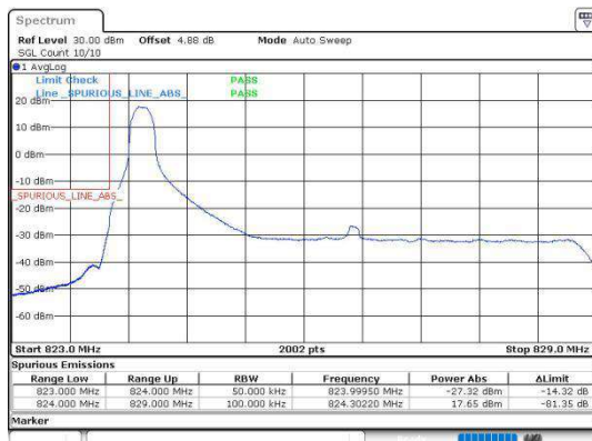
Band5_5MHz_QPSK_20425_1RB#0
