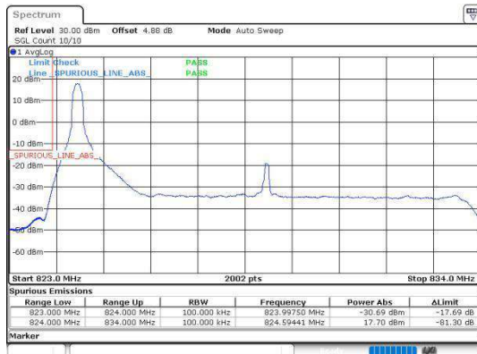
Band5_10MHz_QPSK_20450_50RB#0
