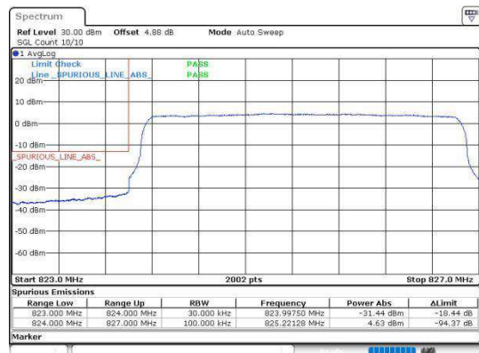
Band5_3MHz_16QAM_20415_15RB#0
