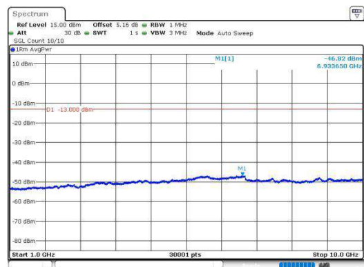
EDGE850-251-5-1000~10000MHz-PASS
