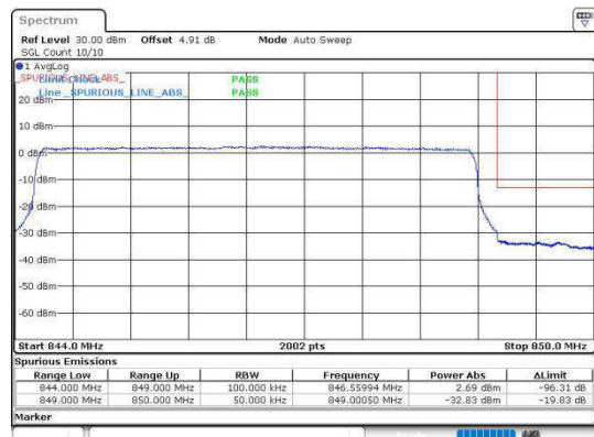
Band5_5MHz_16QAM_20625_25RB#0
