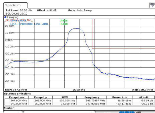
Band5_1.4MHz_16QAM_20643_1RB#5
