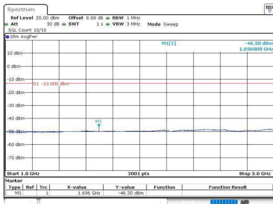
Band5_1.4MHz_16QAM_20643_1RB#0_1000~3000
