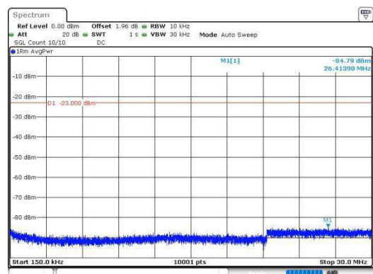
EDGE850-189-5-0.15~30MHz-PASS
