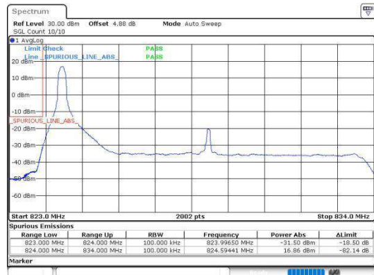
Band5_10MHz_16QAM_20450_50RB#0
