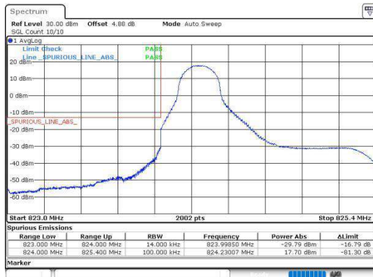
Band5_1.4MHz_QPSK_20407_6RB#0
