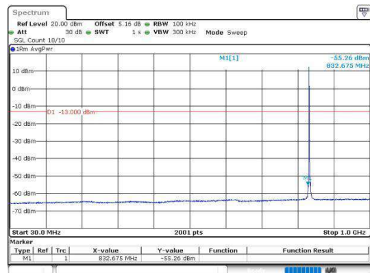
Band5_1.4MHz_16QAM_20525_1RB#0_30~1000
