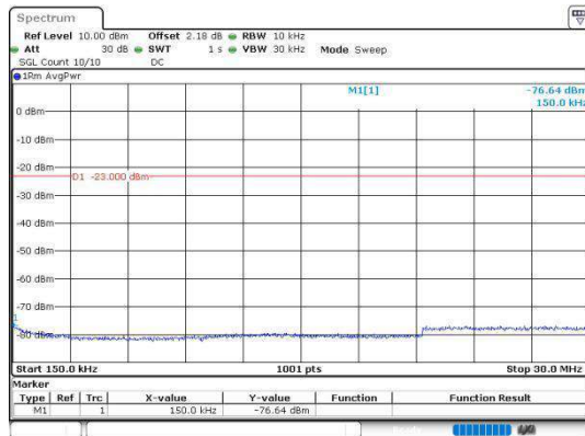
Band5_1.4MHz_16QAM_20407_1RB#0_1000~3000
