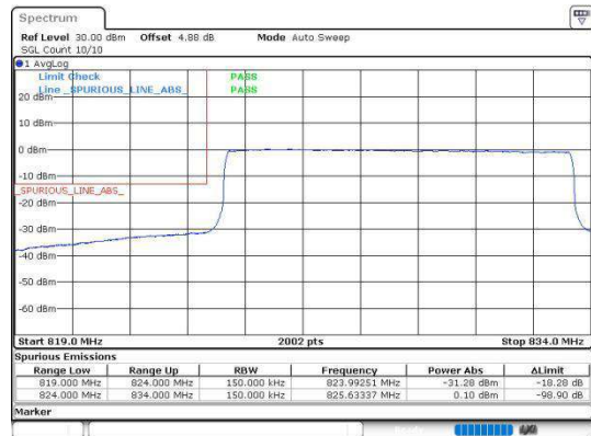
Band5_10MHz_64QAM_20600_50RB#0
