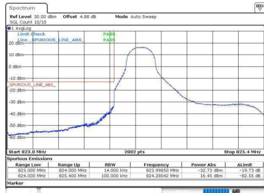
Band5_1.4MHz_16QAM_20407_6RB#0
