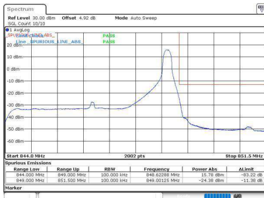
Band5_5MHz_64QAM_20625_1RB#24
