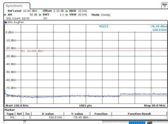
Band5_3MHz_QPSK_20525_1RB#0_0.15~30
