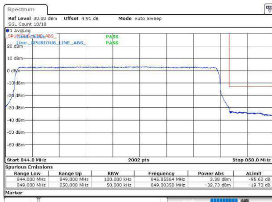
Band5_5MHz_QPSK_20625_25RB#0
