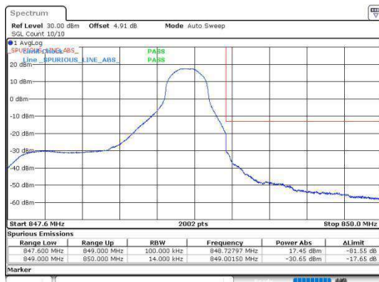
Band5_1.4MHz_QPSK_20643_1RB#5
