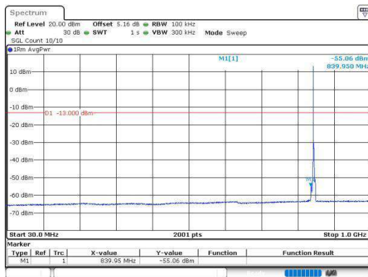
Band5_3MHz_QPSK_20635_1RB#0_30~1000
