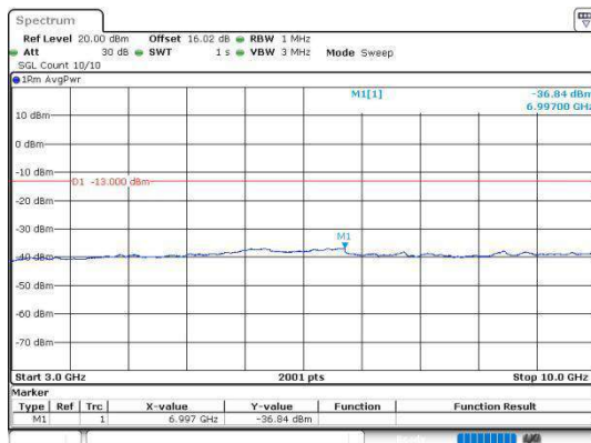
Band5_3MHz_QPSK_20415_1RB#0_3000~10000
