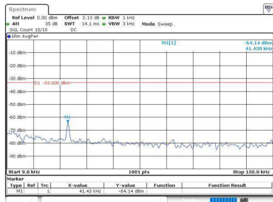
Band5_3MHz_16QAM_20415_1RB#0_0.009~0.15
