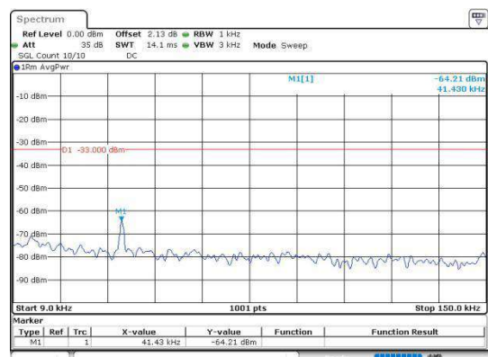
Band5_1.4MHz_16QAM_20407_1RB#0_0.009~0.15
