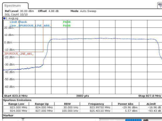
Band5_3MHz_QPSK_20415_15RB#0
