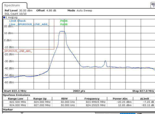
Band5_3MHz_64QAM_20415_1RB#0
