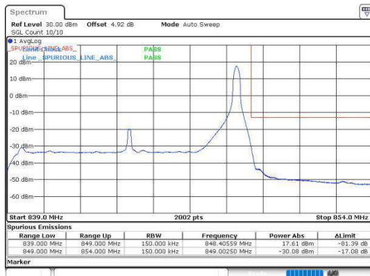
Band5_10MHz_64QAM_20600_1RB#49
