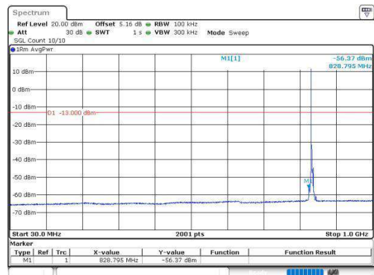
Band5_3MHz_16QAM_20525_1RB#0_30~1000
