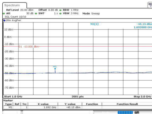
Band5_3MHz_16QAM_20635_1RB#0_1000~3000
