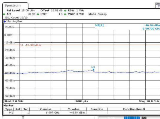
Band5_5MHz_64QAM_20425_1RB#0_3000~10000
