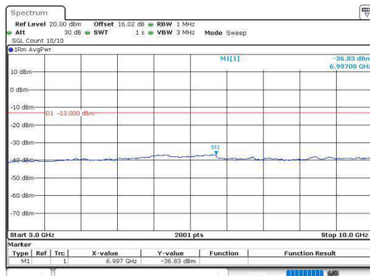
Band5_5MHz_QPSK_20425_1RB#0_3000~10000
