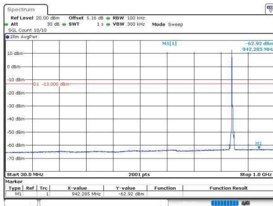
Band5_5MHz_QPSK_20625_1RB#0_30~1000
