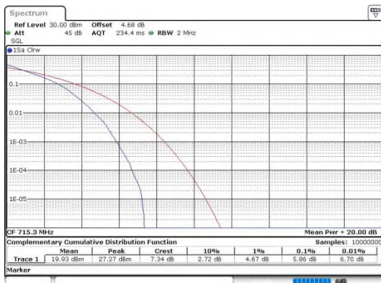
Band12-1.4MHz-QPSK-23173-6RB#0-PASS
