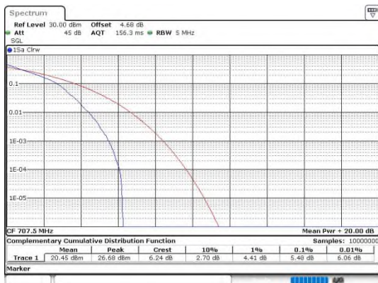
Band12-3MHz-QPSK-23095-1RB#0-PASS
