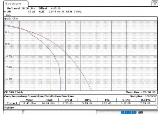
Band12-1.4MHz-16QAM-23017-6RB#0-PASS
