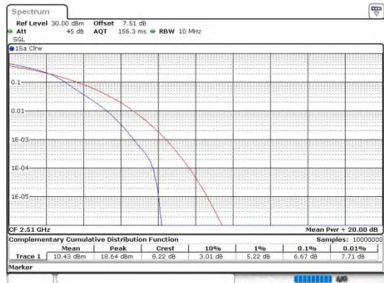
Band7-20MHz-16QAM-20850-100RB#0-PASS
