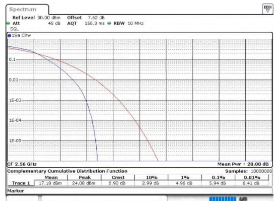
Band7-20MHz-16QAM-21350-100RB#0-PASS
