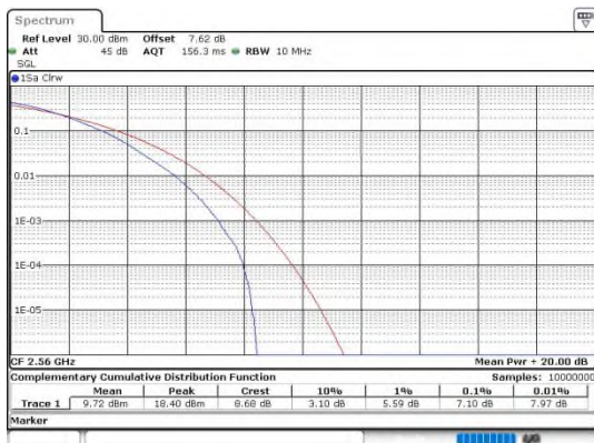
Band7-20MHz-64QAM-21350-1RB#0-PASS
