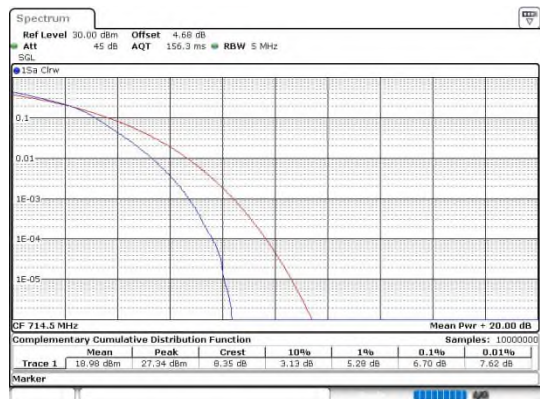
Band12-3MHz-16QAM-23165-15RB#0-PASS
