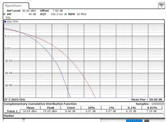
Band7-15MHz-64QAM-21375-75RB#0-PASS
