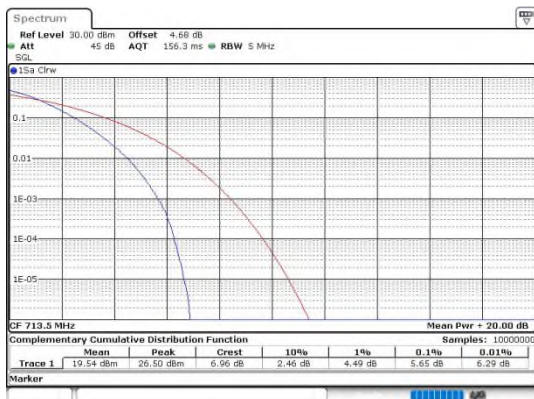
Band12-5MHz-QPSK-23155-25RB#0-PASS
