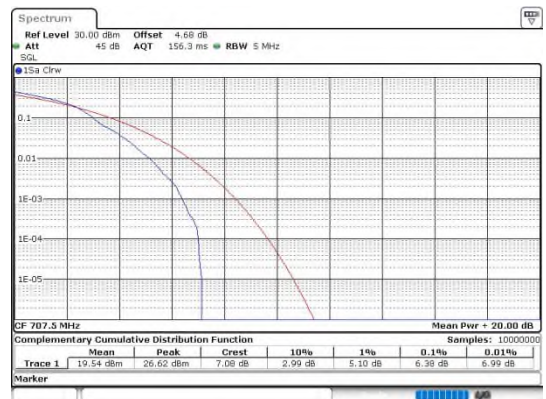
Band12-3MHz-16QAM-23095-1RB#0-PASS
