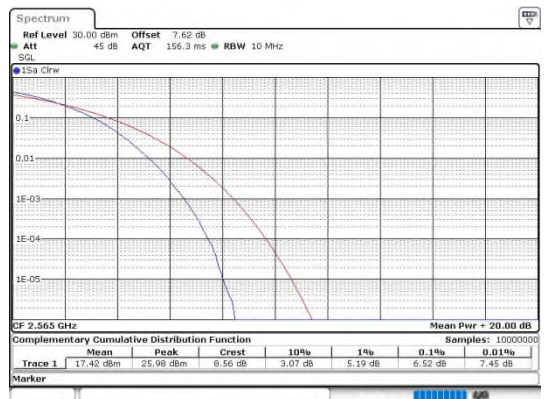
Band7-10MHz-64QAM-21400-50RB#0-PASS
