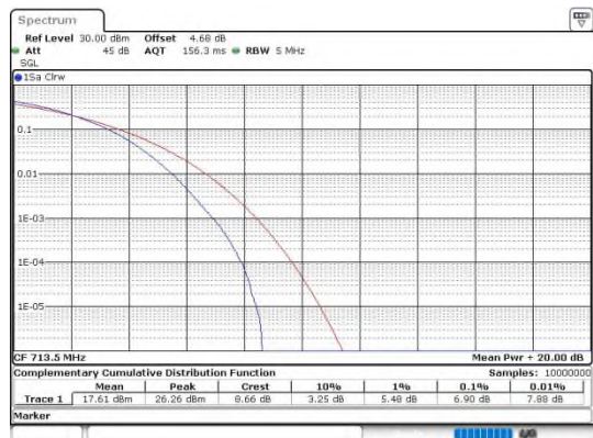
Band12-5MHz-64QAM-23155-25RB#0-PASS
