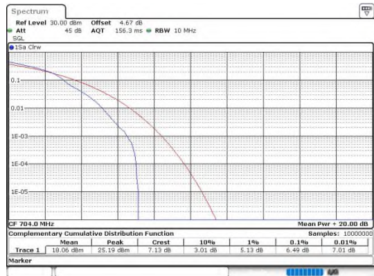
Band12-10MHz-16QAM-23060-50RB#0-PASS
