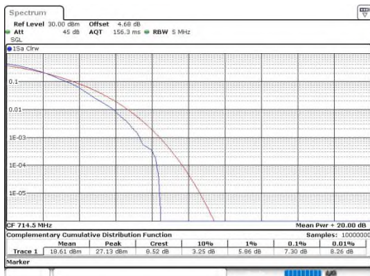
Band12-3MHz-64QAM-23165-1RB#0-PASS
