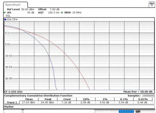
Band7-20MHz-16QAM-21350-1RB#0-PASS
