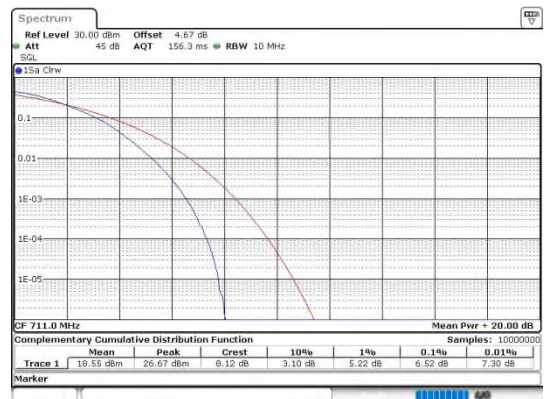
Band12-10MHz-16QAM-23130-50RB#0-PASS
