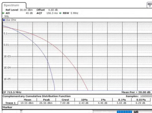
Band17-5MHz-QPSK-23825-25RB#0-PASS
