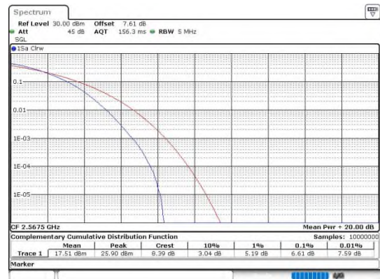
Band7-5MHz-64QAM-21425-25RB#0-PASS
