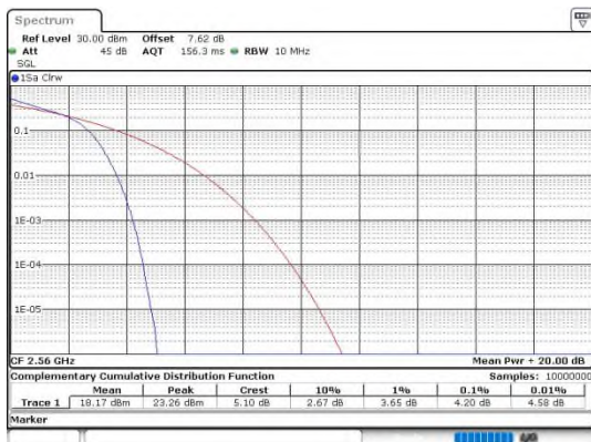
Band7-20MHz-QPSK-21350-100RB#0-PASS
