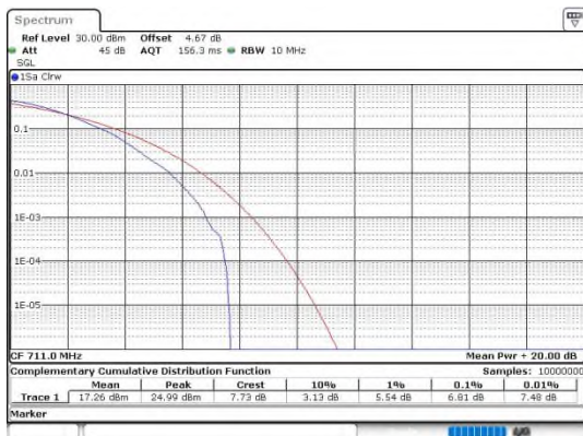
Band12-10MHz-64QAM-23130-1RB#0-PASS
