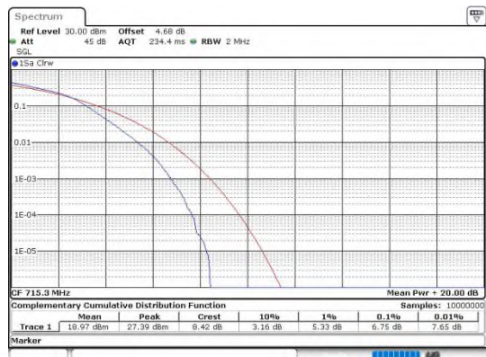
Band12-1.4MHz-16QAM-23173-6RB#0-PASS
