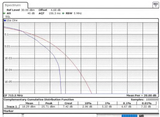
Band12-5MHz-16QAM-23155-25RB#0-PASS
