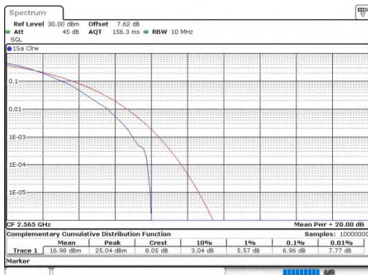
Band7-10MHz-64QAM-21400-1RB#0-PASS
