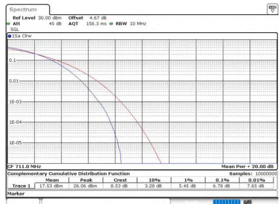
Band12-10MHz-64QAM-23130-50RB#0-PASS
