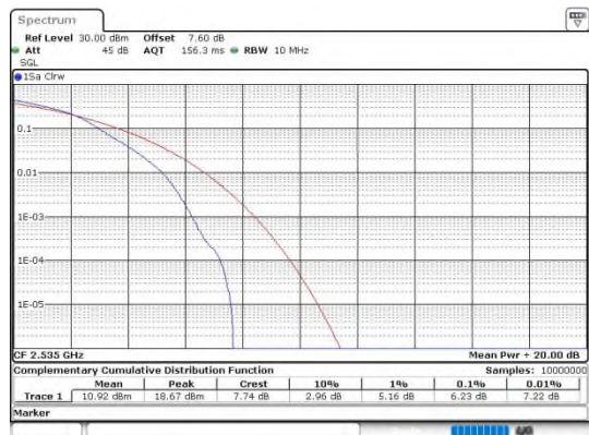
Band7-20MHz-16QAM-21100-1RB#0-PASS
