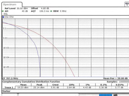
Band12-5MHz-QPSK-23095-1RB#0-PASS
