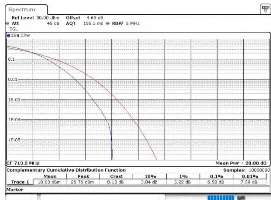
Band17-5MHz-16QAM-23825-25RB#0-PASS
