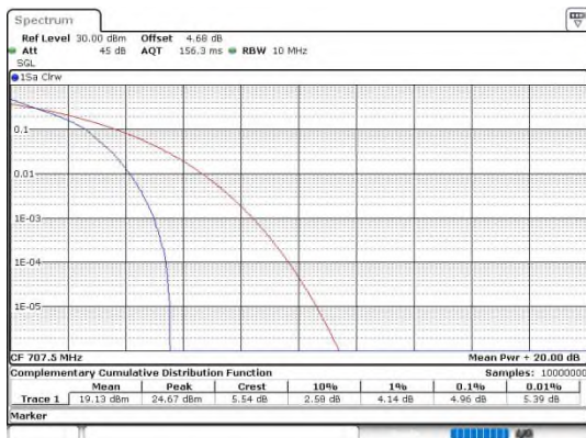
Band12-10MHz-QPSK-23095-1RB#0-PASS
