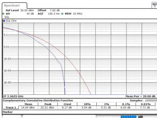
Band7-15MHz-64QAM-21375-1RB#0-PASS
