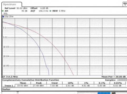
Band12-3MHz-QPSK-23165-15RB#0-PASS
