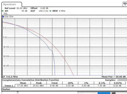
Band12-5MHz-64QAM-23155-1RB#0-PASS
