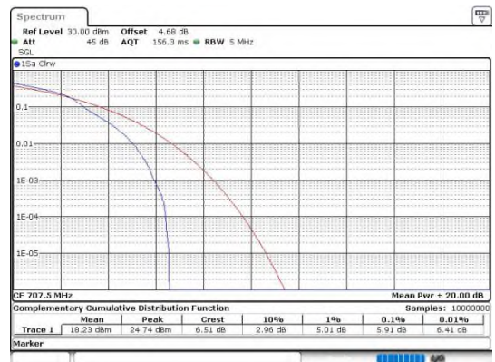
Band12-5MHz-16QAM-23095-1RB#0-PASS
