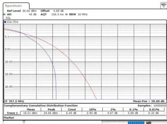
Band12-10MHz-16QAM-23095-1RB#0-PASS
