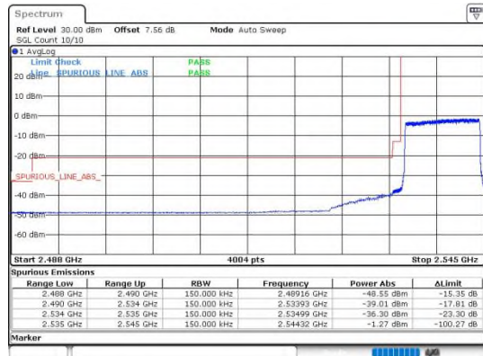
Band41_10MHz_64QAM_40090_50RB#0
