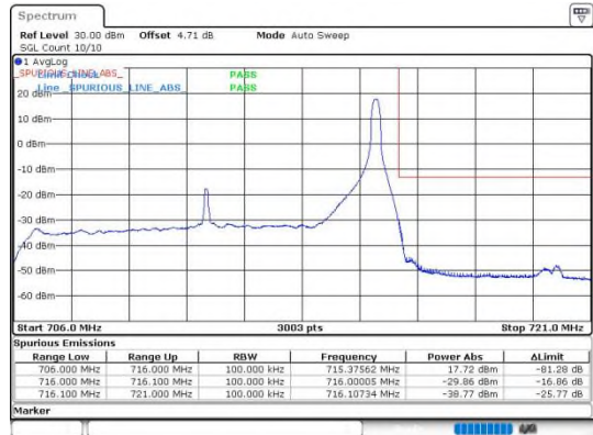
Band17_10MHz_16QAM_23800_50RB#0
