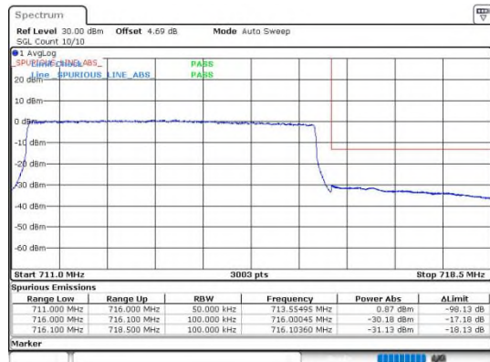
Band17_10MHz_16QAM_23780_1RB#0
