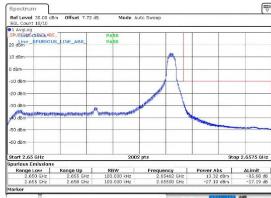
Band41_5MHz_16QAM_41215_1RB#24
