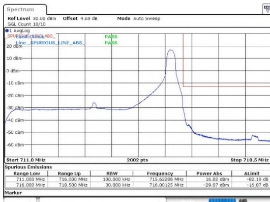
Band12_5MHz_64QAM_23155_1RB#24
