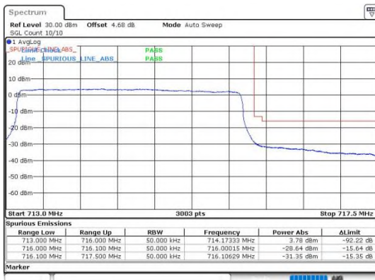
Band12_5MHz_QPSK_23035_1RB#0
