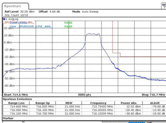
Band12_1.4MHz_QPSK_23173_1RB#5
