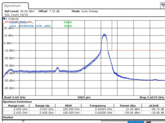
Band41_5MHz_64QAM_41215_1RB#24
