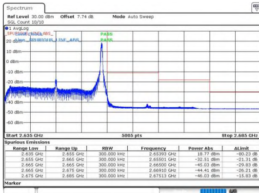
Band41_20MHz_64QAM_41140_1RB#99
