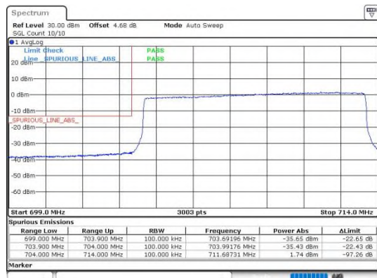
Band17_10MHz_16QAM_23780_50RB#0
