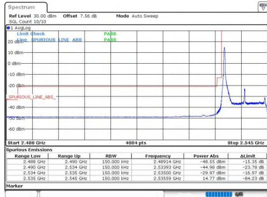
Band41_10MHz_QPSK_40090_50RB#0
