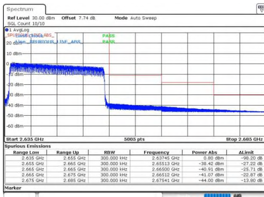
Band41_20MHz_16QAM_41140_100RB#0
