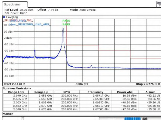
Band41_15MHz_64QAM_41165_1RB#74
