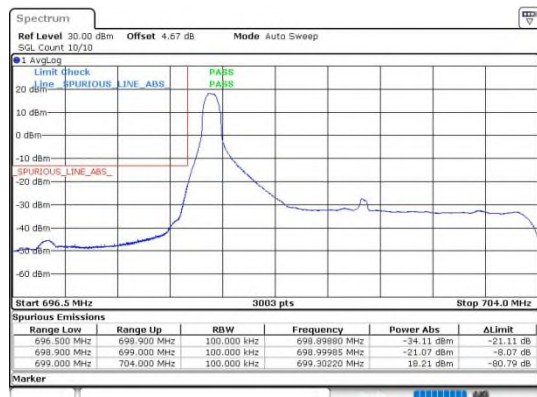
Band12_5MHz_16QAM_23035_1RB#0
