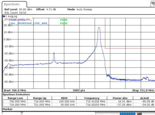
Band17_10MHz_64QAM_23800_1RB#49
