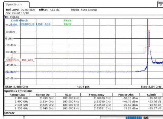
Band41_5MHz_16QAM_40065_25RB#0
