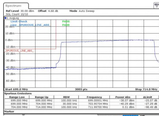
Band17_10MHz_64QAM_23780_50RB#0
