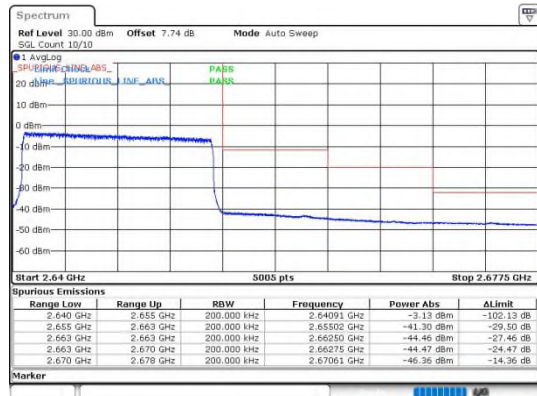
Band41_15MHz_64QAM_41165_75RB#0
