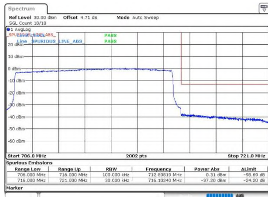
Band12_10MHz_64QAM_23130_50RB#0
