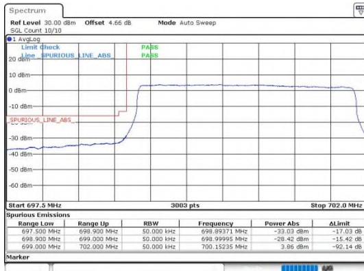
Band12_3MHz_QPSK_23025_15RB#0
