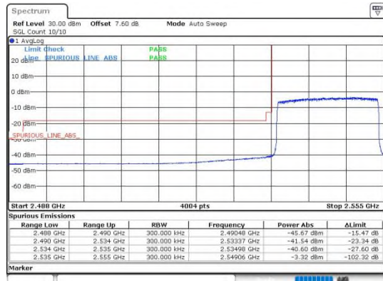
Band41_20MHz_64QAM_40140_100RB#0
