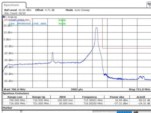
Band12_10MHz_64QAM_23130_1RB#49
