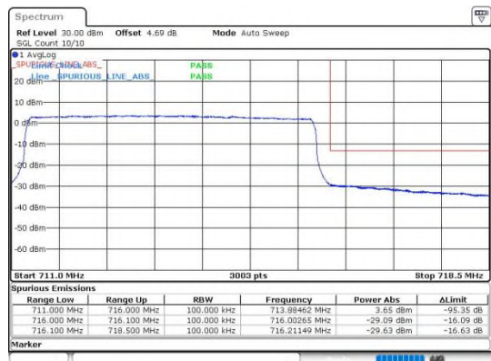
Band12_5MHz_16QAM_23155_25RB#0
