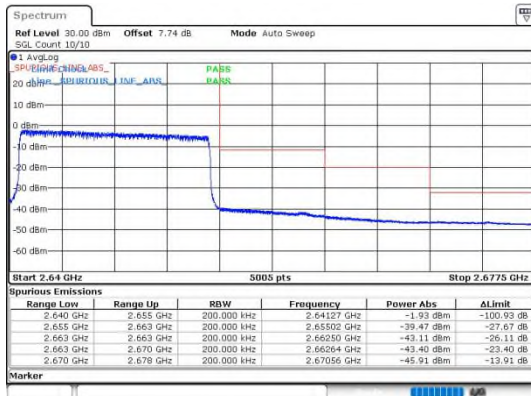
Band41_15MHz_16QAM_41165_75RB#0
