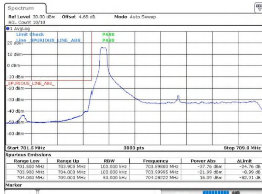
Band17_5MHz_QPSK_23755_25RB#0
