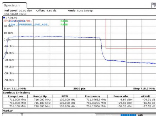
Band12_5MHz_QPSK_23155_25RB#0
