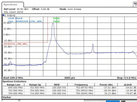
Band17_10MHz_QPSK_23780_50RB#0
