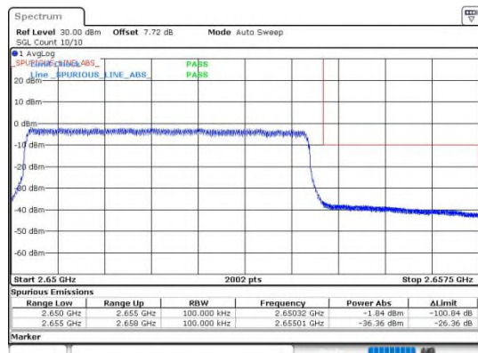
Band41_5MHz_64QAM_41215_25RB#0
