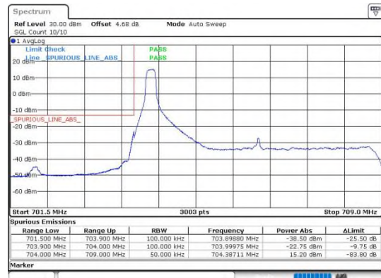
Band17_5MHz_16QAM_23755_25RB#0
