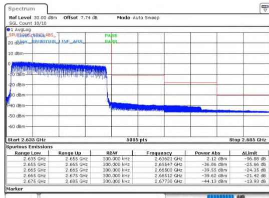
Band41_20MHz_64QAM_41140_100RB#0
