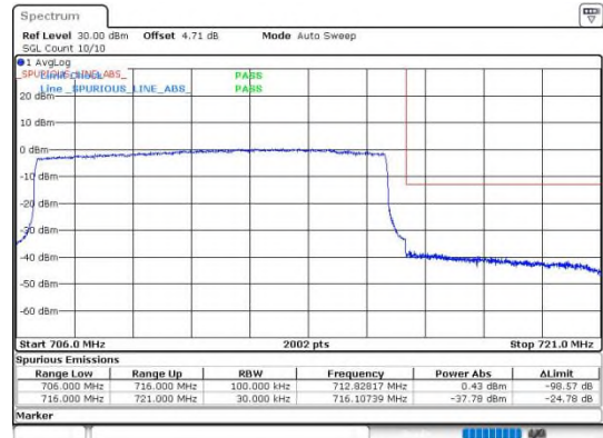
Band17_10MHz_64QAM_23800_50RB#0
