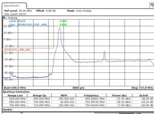
Band17_10MHz_64QAM_23780_1RB#0
