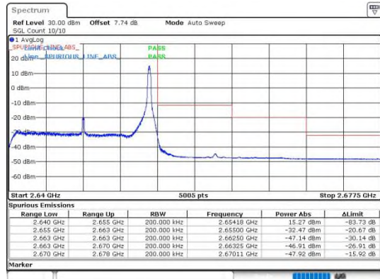
Band41_15MHz_QPSK_41165_75RB#0
