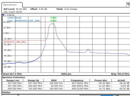
Band12_3MHz_64QAM_23025_1RB#0
