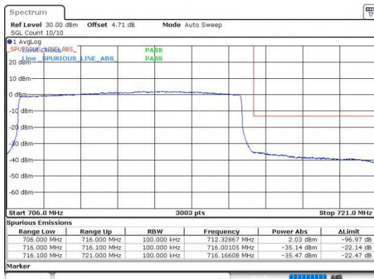
Band17_10MHz_QPSK_23800_50RB#0
