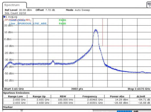
Band41_5MHz_QPSK_41215_1RB#24
