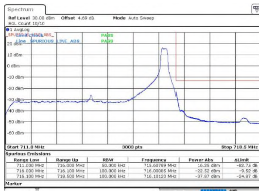
Band17_5MHz_QPSK_23825_1RB#24
