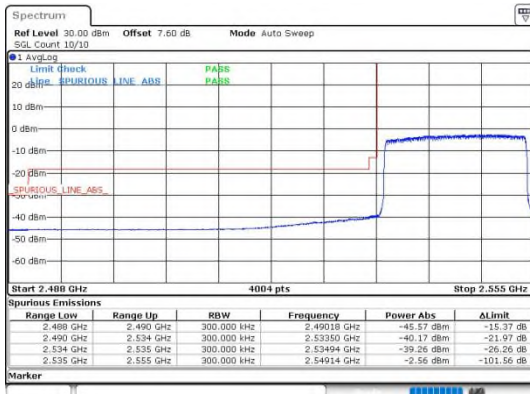
Band41_20MHz_16QAM_40140_100RB#0
