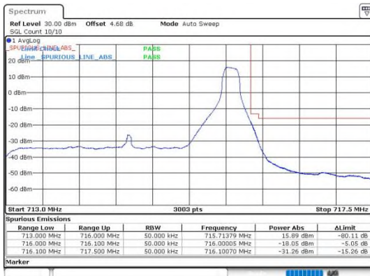
Band12_3MHz_QPSK_23165_15RB#0
