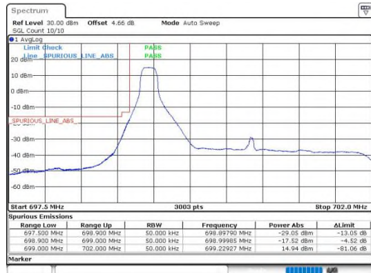
Band12_3MHz_16QAM_23025_15RB#0
