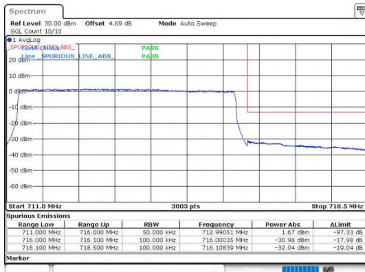
Band17_10MHz_QPSK_23780_1RB#0
