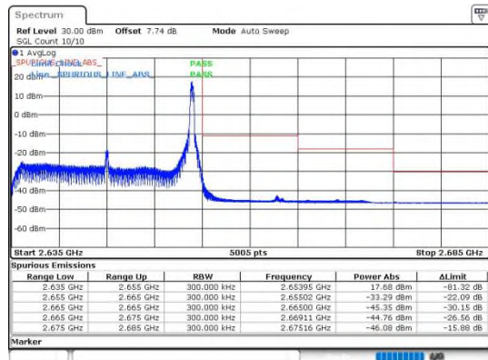
Band41_20MHz_QPSK_41140_100RB#0
