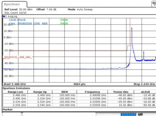
Band41_10MHz_64QAM_40090_1RB#0
