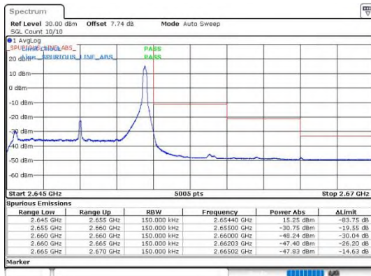
Band41_10MHz_64QAM_41190_1RB#49
