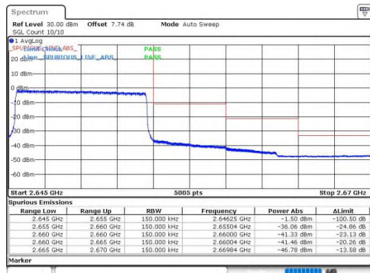
Band41_10MHz_64QAM_41190_50RB#0
