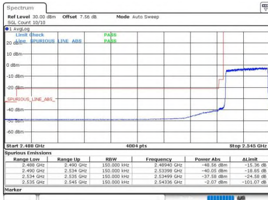
Band41_10MHz_16QAM_40090_50RB#0
