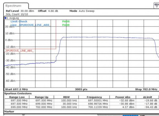
Band12_3MHz_64QAM_23025_15RB#0
