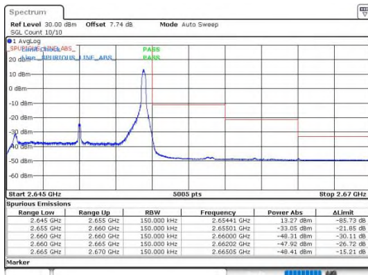
Band41_10MHz_16QAM_41190_50RB#0
