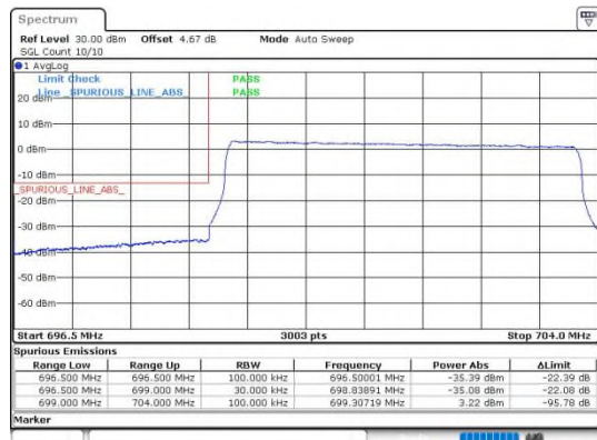
Band12_5MHz_64QAM_23155_25RB#0
