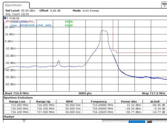
Band12_3MHz_16QAM_23165_15RB#0
