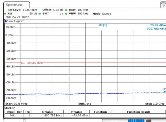
Band41_10MHz_QPSK_40090_1RB#0_30~1000
