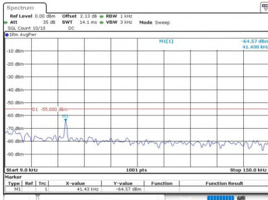
Band41_20MHz_64QAM_40140_1RB#0_0.009~0.15
