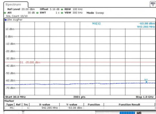
Band41_20MHz_QPSK_40590_1RB#0_30~1000
