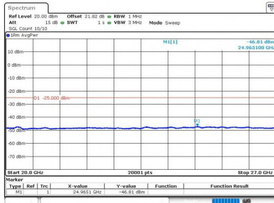
Band41_20MHz_QPSK_41140_1RB#0_20000~27000
