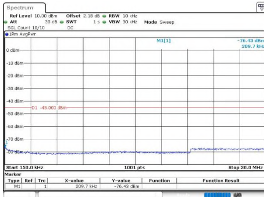
Band41_20MHz_QPSK_40590_1RB#0_0.15~30
