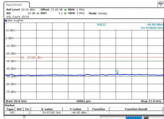
Band41_20MHz_64QAM_40140_1RB#0_0.15~30
