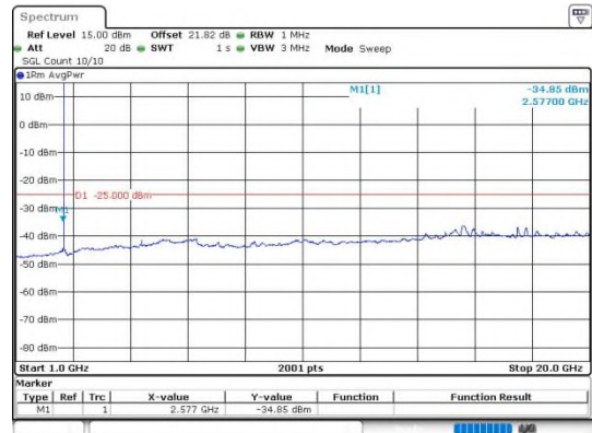
Band41_5MHz_16QAM_40590_1RB#0_1000~20000
