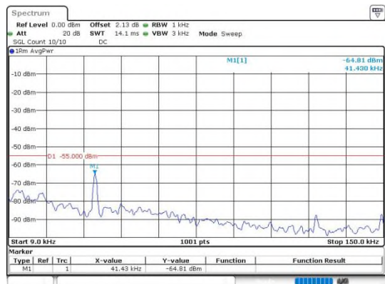
Band41_5MHz_16QAM_41215_1RB#0_0.009~0.15
