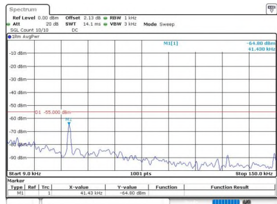
Band41_15MHz_16QAM_40590_1RB#0_0.009~0.15
