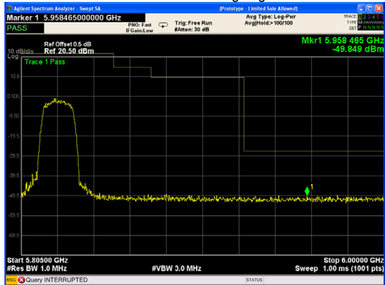
802.11a U-NII-3 Band edge-right side
