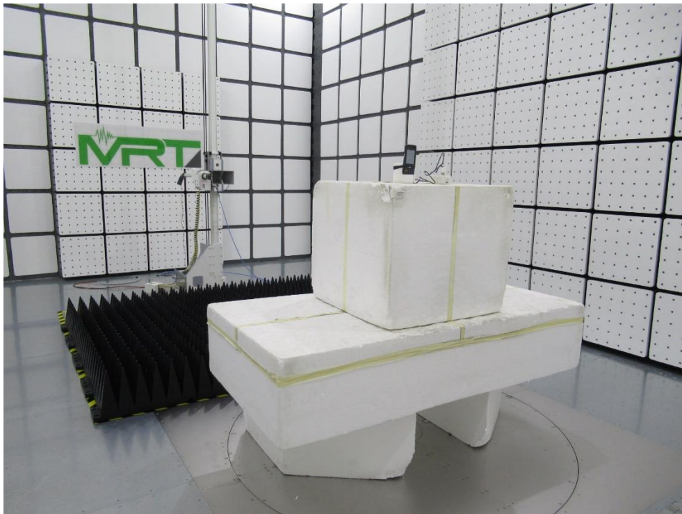
Radiated Emission Test Setup for above 1GHz
