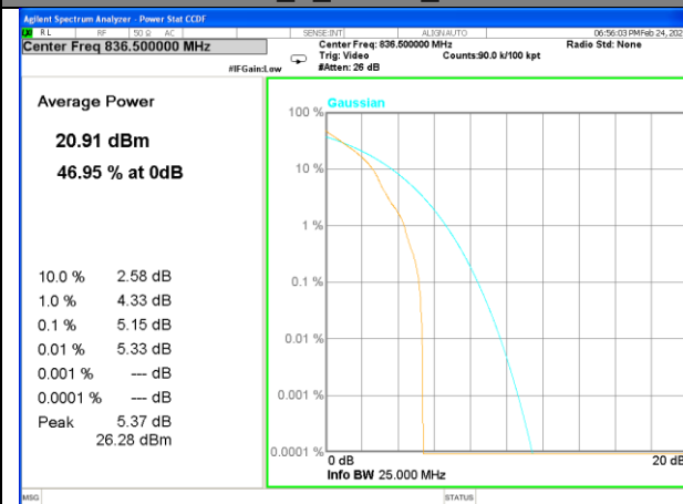
Band 5_1_QPSK_Middle
