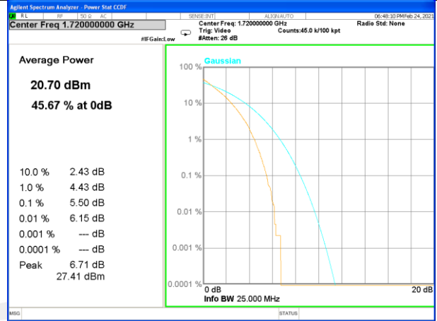
Band 4_100_Q16_Low
