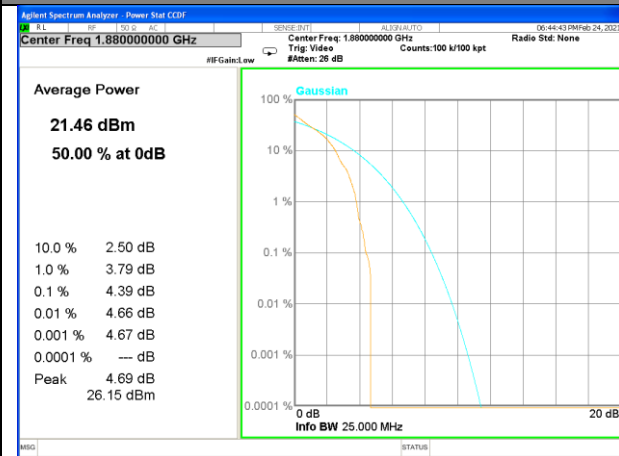
Band 2_1_QPSK_Middle
