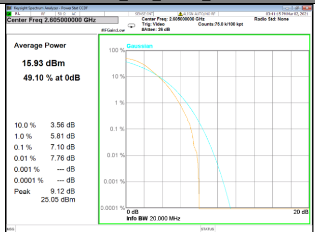
Band 41_100_QPSK_Middle
