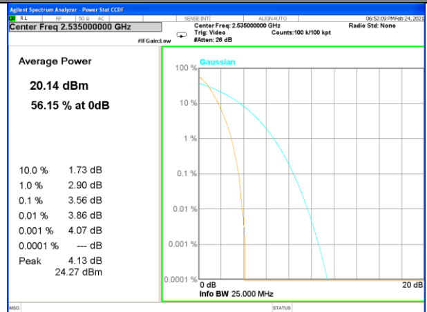
Band 7_100_QPSK_Middle
