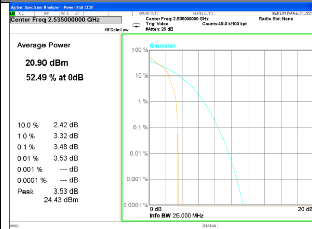
Band 7_1_QPSK_Middle
