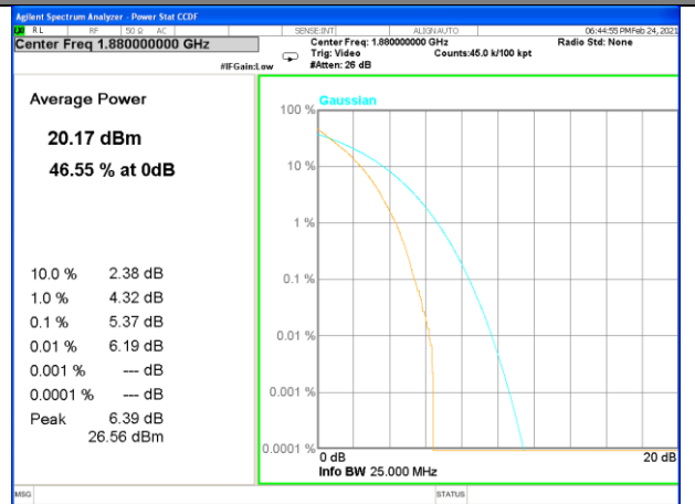
Band 2_100_QPSK_Middle
