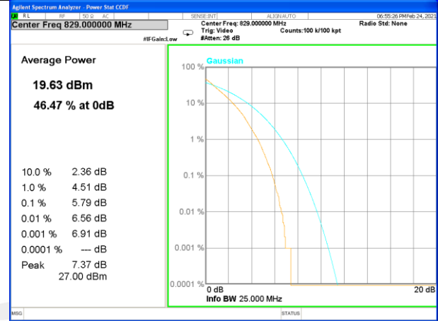
Band 5_50_Q16_Low
