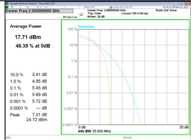
Band 41_1_QPSK_Middle
