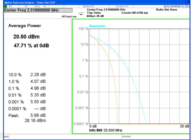
Band 7_100_Q16_Low
