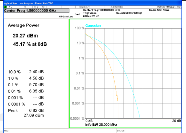
Band 2_100_Q16_Low
