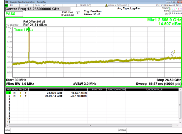
Band 41_10M_QPSK_Middle
