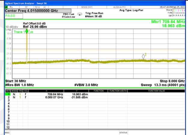
Band 17_10M_16QAM_High
