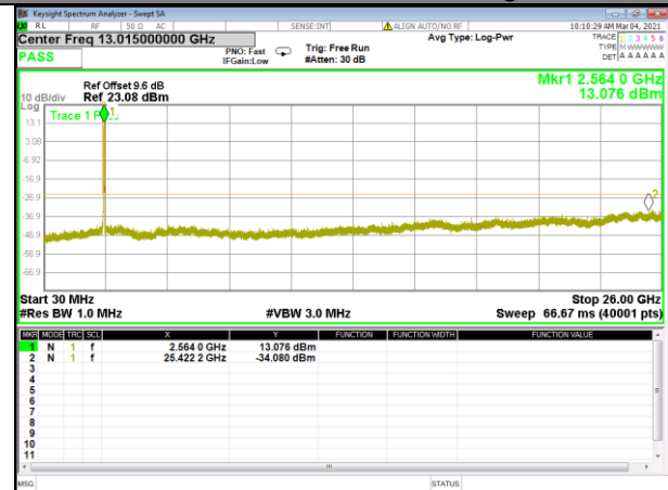
Band 7_20M_16QAM_High
