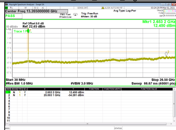
Band 41_15M_QPSK_High
