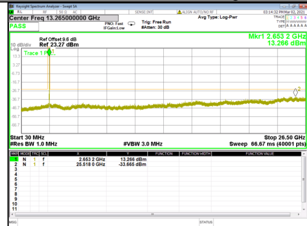
Band 41_10M_QPSK_High
