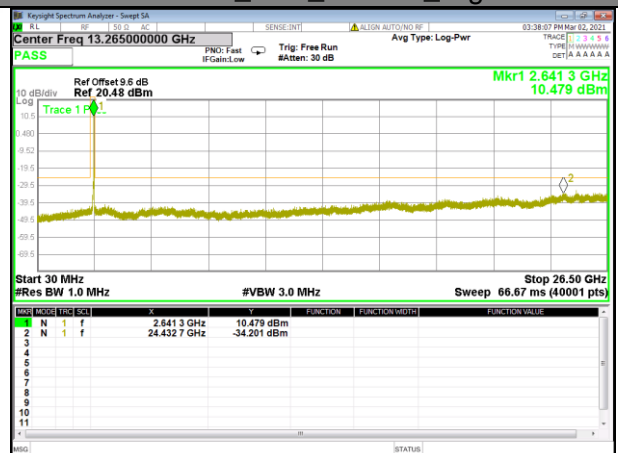
Band 41_20M_16QAM_High
