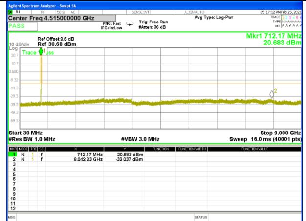
Band 12_5M_16QAM_High
