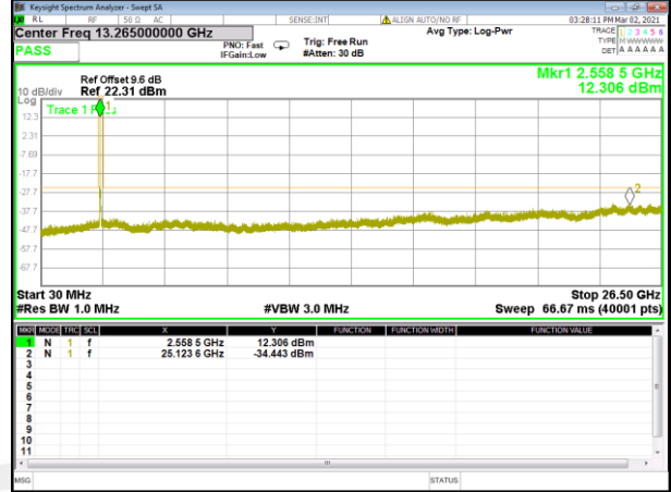
Band 41_15M_16QAM_Middle
