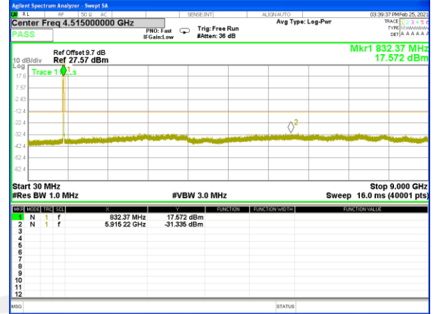
Band 5_10M_16QAM_Middle
