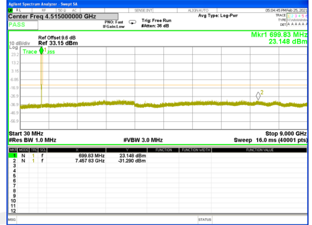
Band 12_3M_16QAM_Middle
