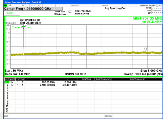
Band 17_10M_16QAM_Middle
