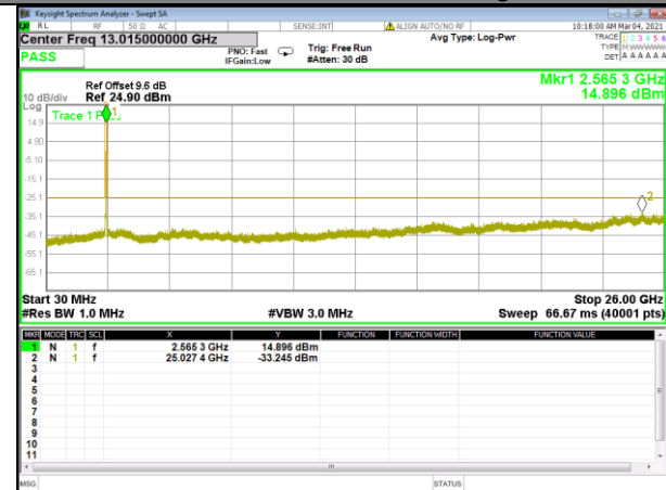
Band 7_15M_QPSK_High
