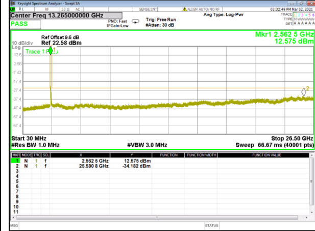
Band 41_20M_QPSK_Middle
