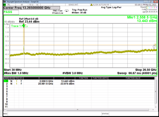
Band 41_10M_16QAM_Middle
