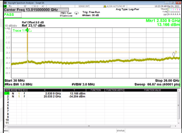
Band 7_15M_16QAM_High
