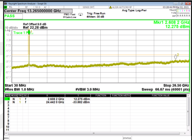
Band 41_15M_16QAM_High
