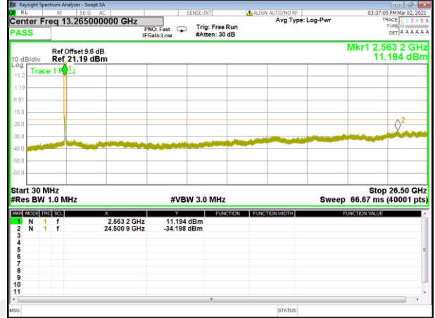
Band 41_20M_16QAM_Middle
