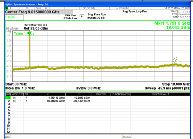
Band 4_5M_16QAM_High
