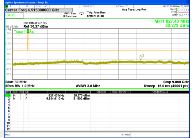
Band 5_5M_16QAM_Middle
