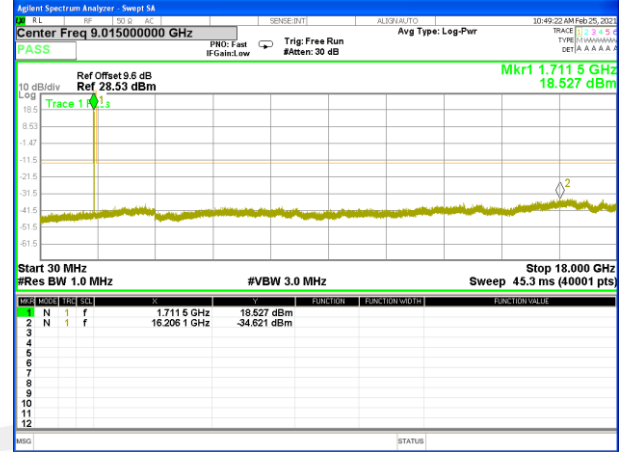
Band 4_5M_16QAM_Middle
