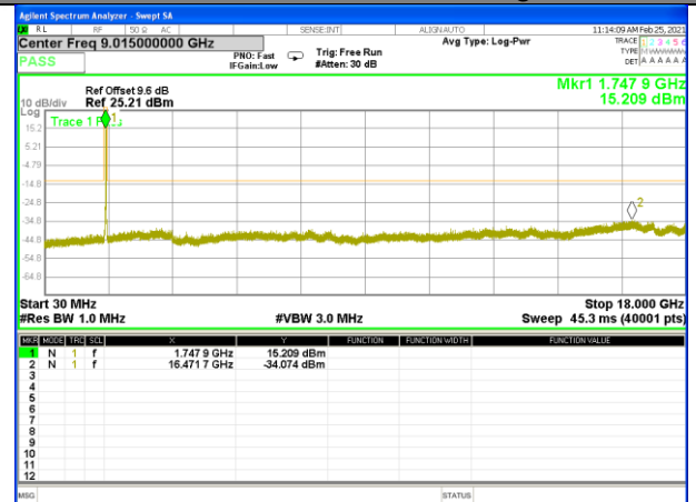
Band 4_15M_16QAM_High
