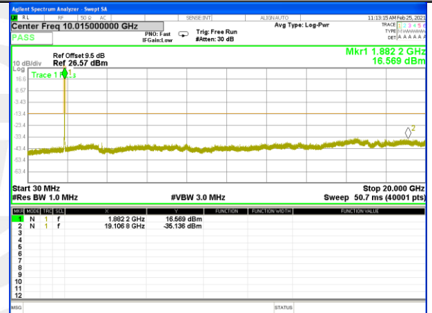
Band 2_10M_16QAM_High
