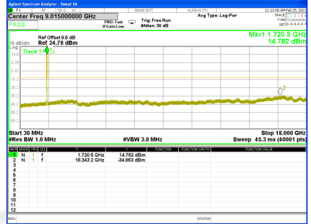
Band 4_15M_16QAM_Middle
