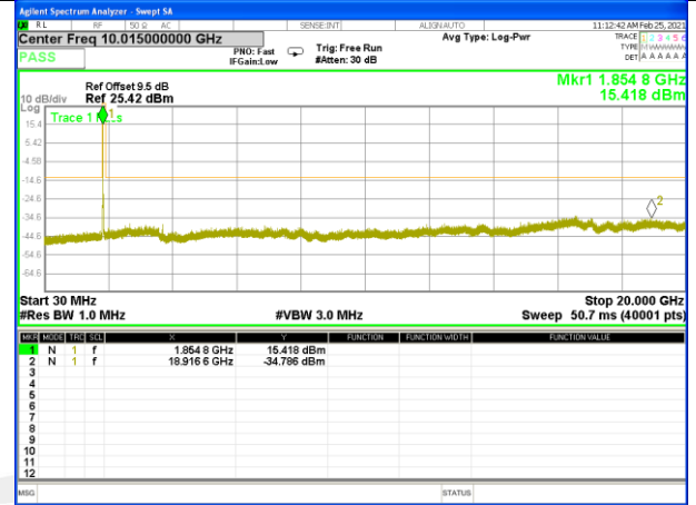
Band 2_10M_16QAM_Middle
