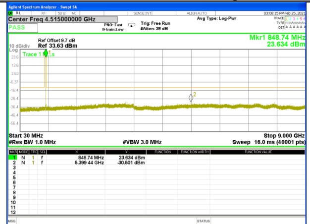
Band 5_1.4M_16QAM_High
