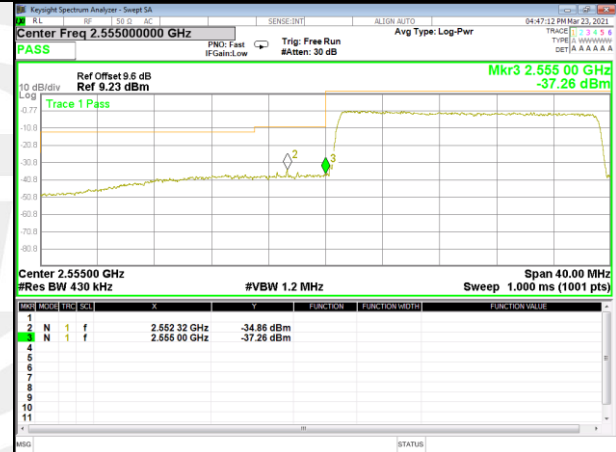
Band 41_20M_16QAM_High_1-RB
