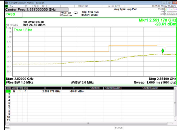
Band 41_15M_QPSK_High_1-RB
