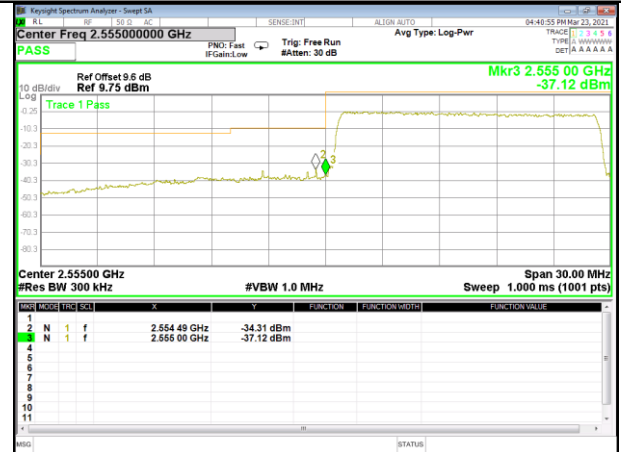
Band 41_15M_16QAM_Low_Full-RB
