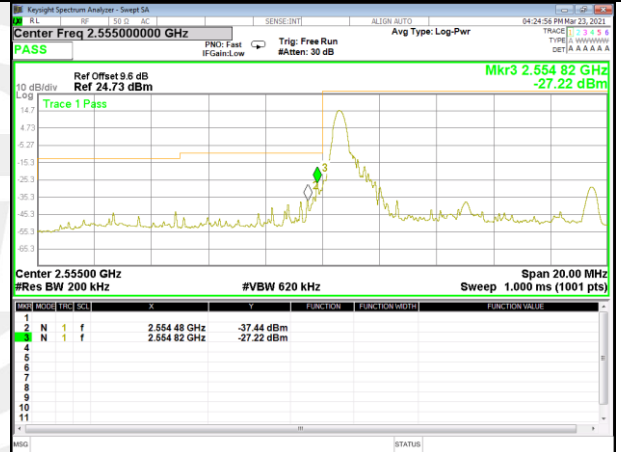
Band 41_10M_QPSK_Low_Full-RB
