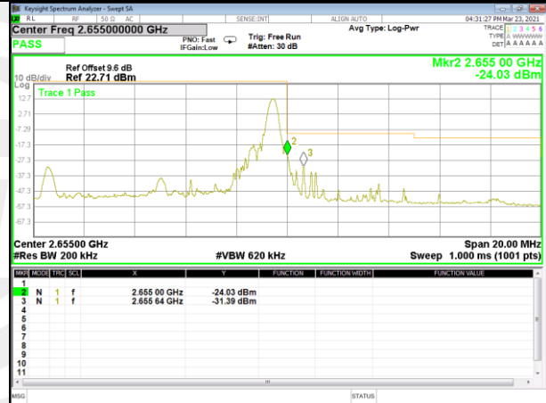
Band 41_10M_16QAM_High_Full-RB
