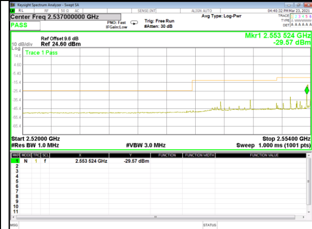
Band 41_15M_16QAM_Low_Full-RB
