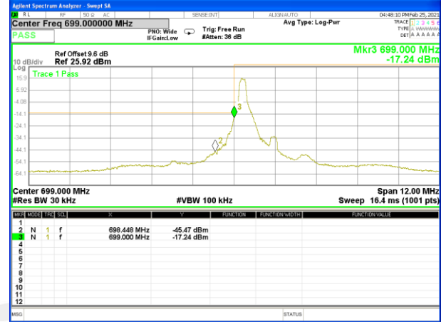
Band12_1.4M_QPSK_Low_Full-RB
