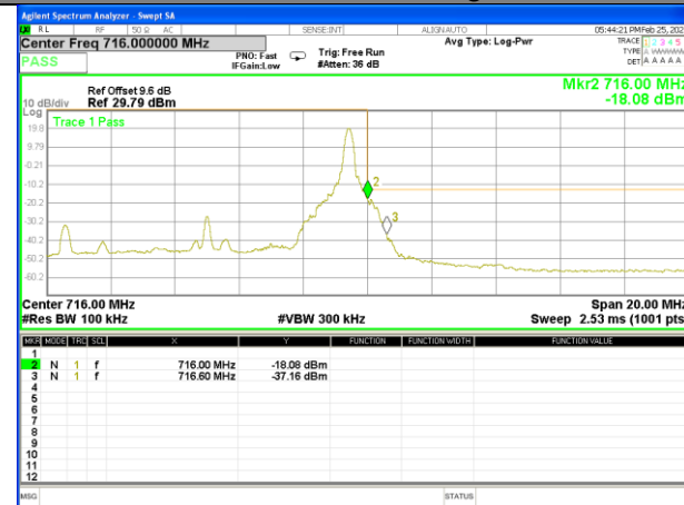
Band17_10M_QPSK_High_1-RB
