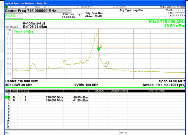
Band12_3M_QPSK_High_Full-RB
