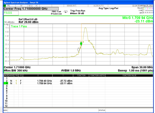
Band 4_15M_16QAM_Low_Full-RB
