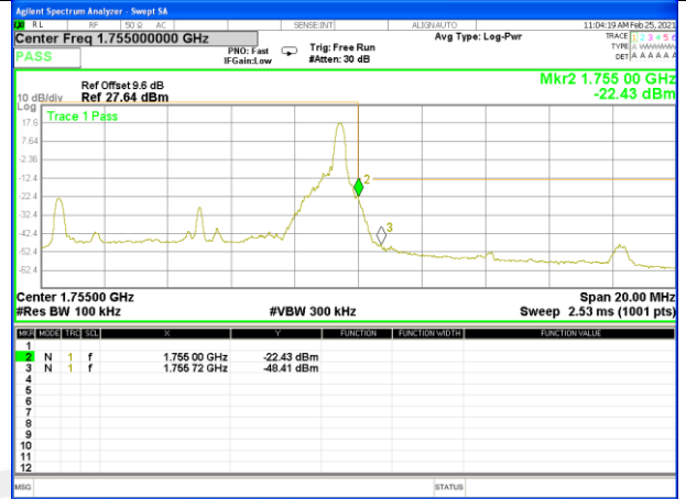
Band 4_10M_16QAM_High_Full-RB
