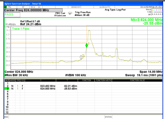
Band 5_3M_QPSK_Low_1-RB
