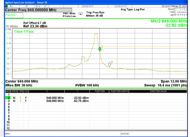
Band 5_1.4M_16QAM_High_Full-RB
