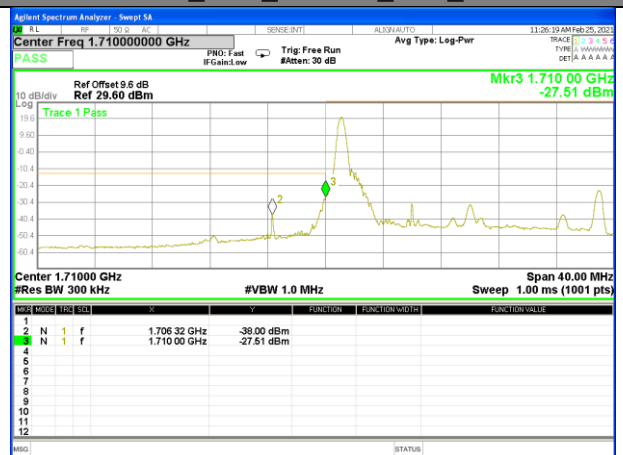
Band 4_20M_16QAM_Low_1-RB
