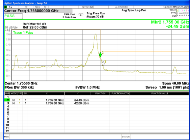
Band 4_20M_QPSK_High_Full-RB
