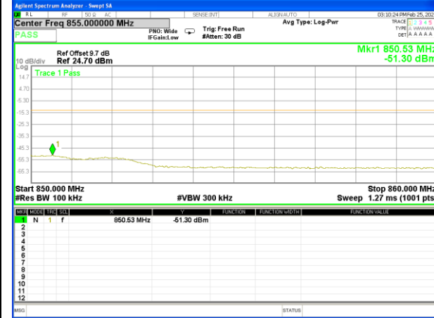
Band 5_1.4M_16QAM_High_Full-RB
