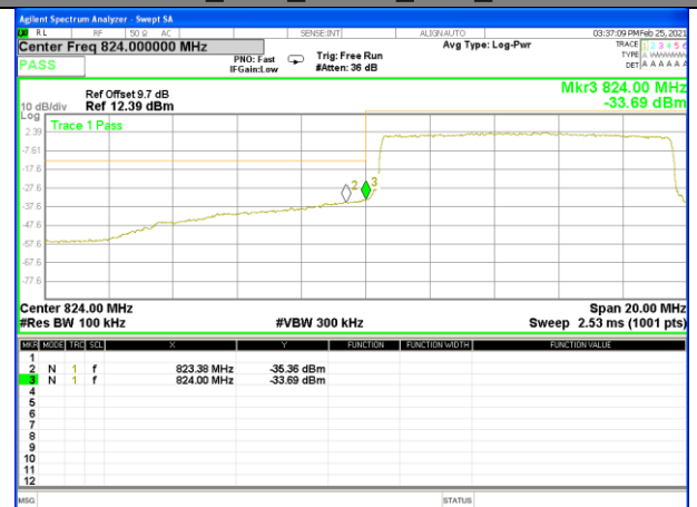
Band 5_10M_QPSK_Low_Full-RB
