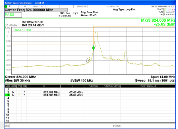
Band 5_3M_16QAM_Low_Full-RB
