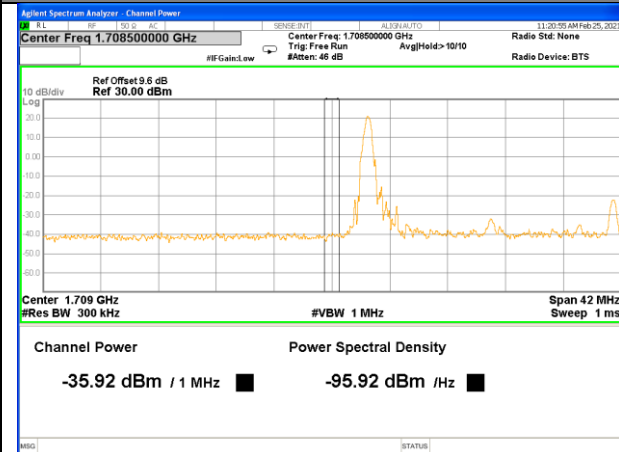
Band 4_20M_QPSK_Low_Full-RB
