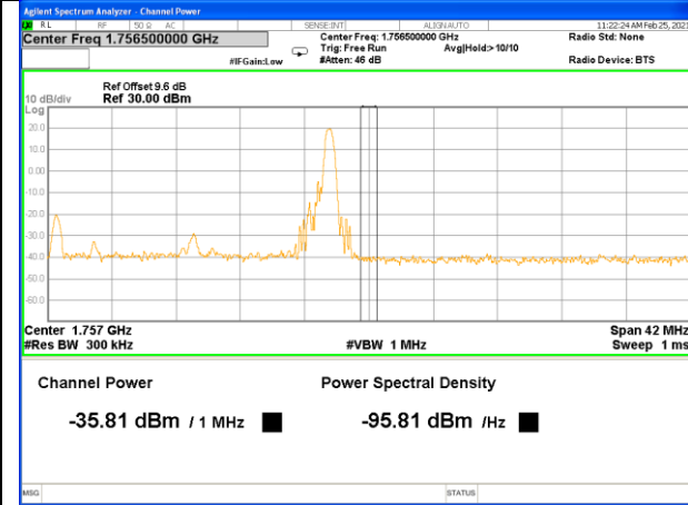
Band 4_20M_QPSK_High_Full-RB
