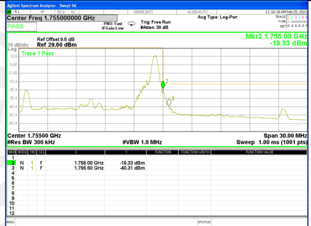
Band 4_15M_QPSK_High_Full-RB
