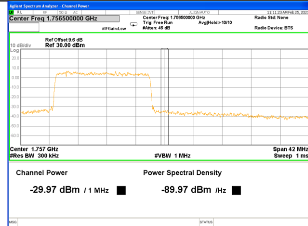
Band 4_15M_QPSK_High_Full-RB
