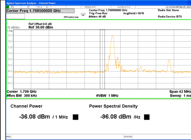
Band 4_15M_16QAM_Low_Full-RB
