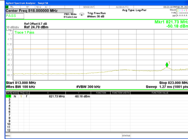
Band 5_3M_16QAM_Low_Full-RB
