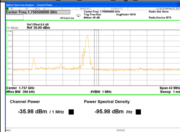
Band 4_15M_16QAM_High_1-RB
