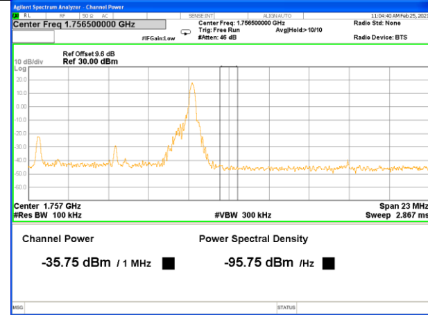
Band 4_10M_16QAM_High_Full-RB
