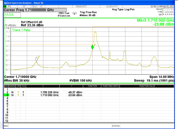
Band 4_3M_16QAM_Low_Full-RB
