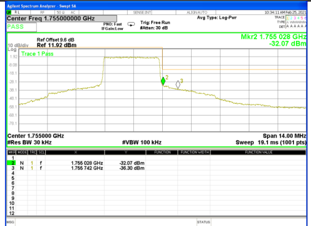
Band 4_3M_QPSK_High_Full-RB
