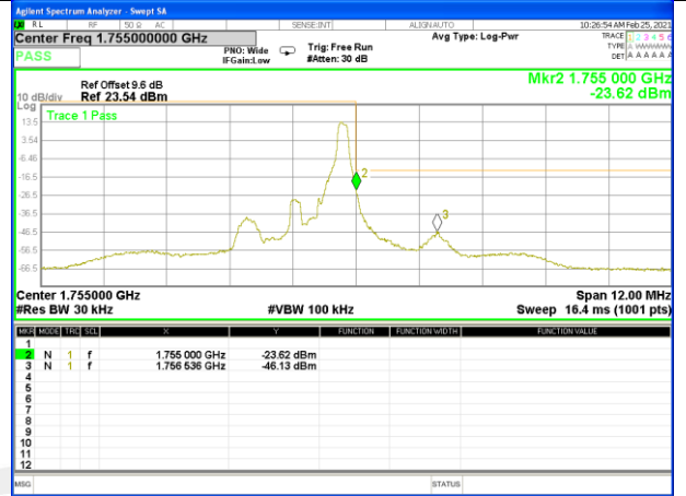
Band 4_1.4M_16QAM_High_Full-RB
