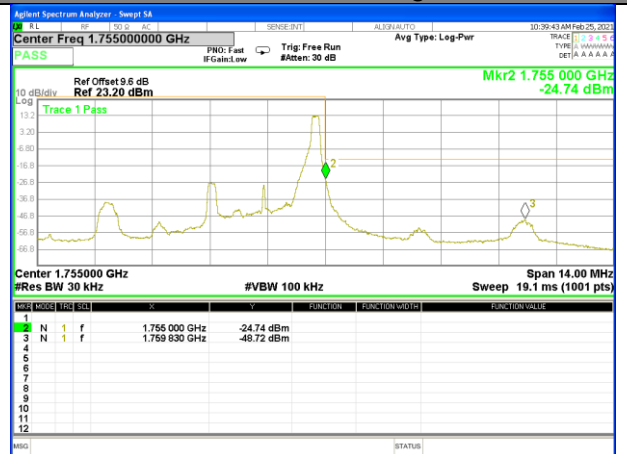
Band 4_3M_16QAM_High_1-RB
