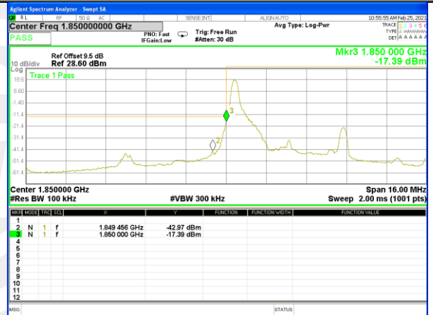
Band 2_5M_QPSK_Low_Full-RB
