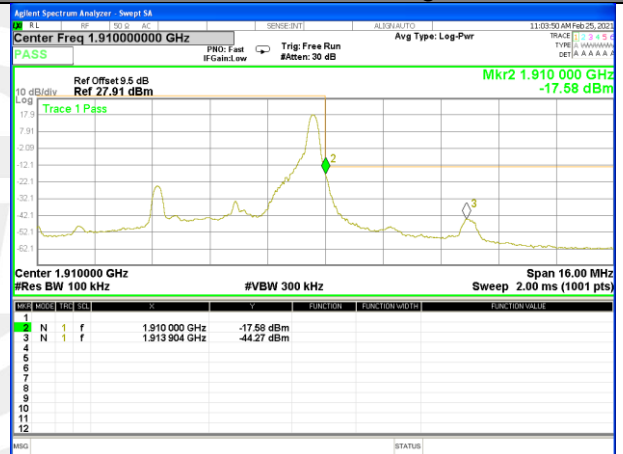
Band 2_5M_16QAM_High_Full-RB
