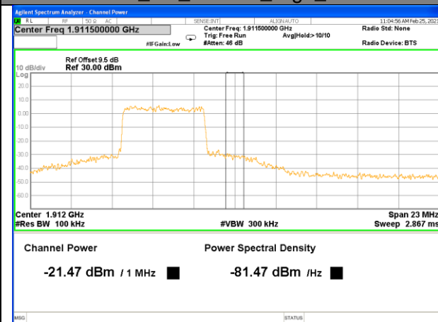
Band 2_5M_16QAM_High_Full-RB
