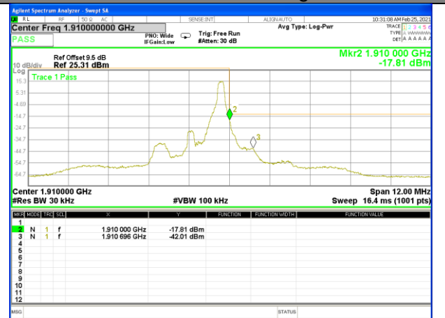
Band 2_1.4M_QPSK_High_1-RB
