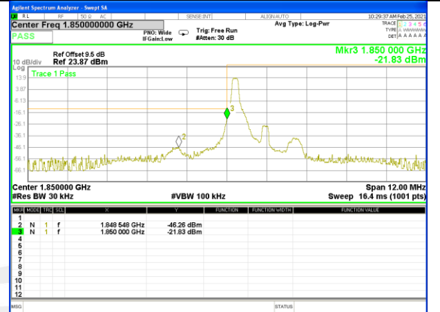
Band 2_1.4M_QPSK_Low_Full-RB
