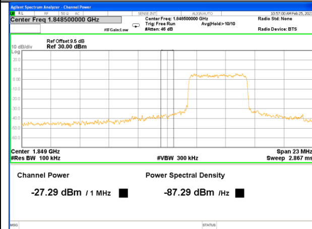
Band 2_5M_QPSK_Low_Full-RB
