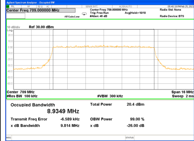
Band 17_10M_QPSK_Middle
