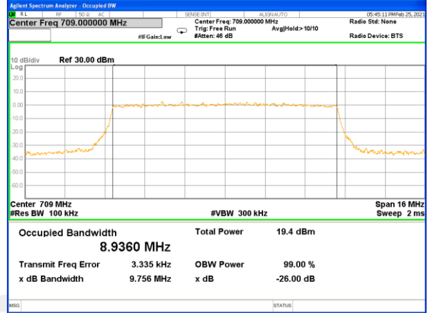
Band 17_10M_16QAM_Middle
