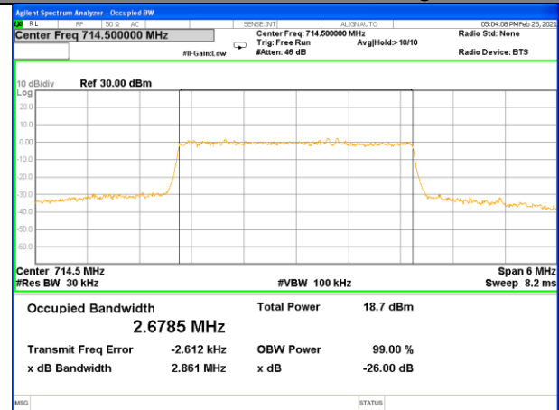
Band 12_3M_16QAM_High
