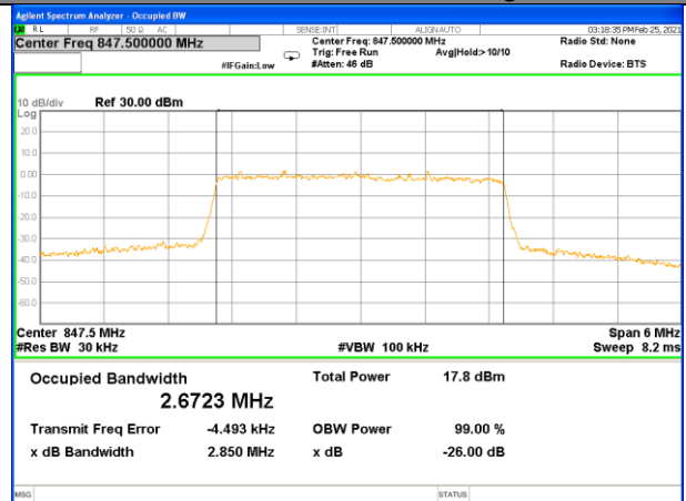
Band 5_3M_16QAM_High
