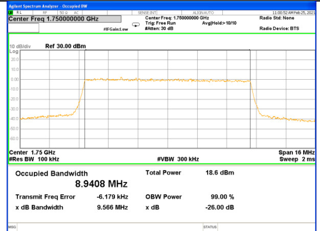
Band 4_10M_16QAM_High
