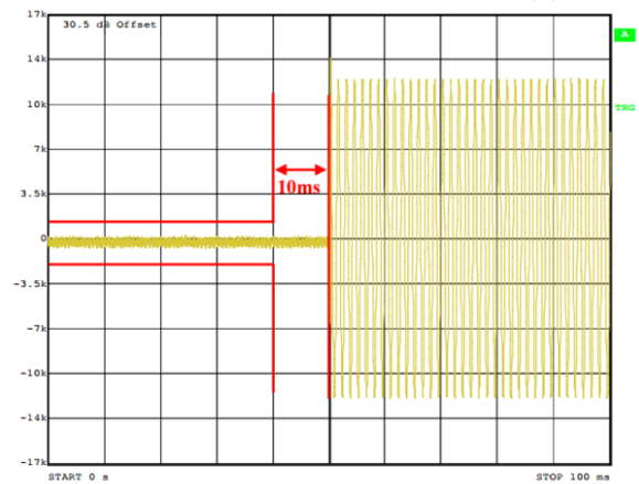
Transmitter Frequency Behavior @ 12.5 KHz Channel Separation-----On – Off
