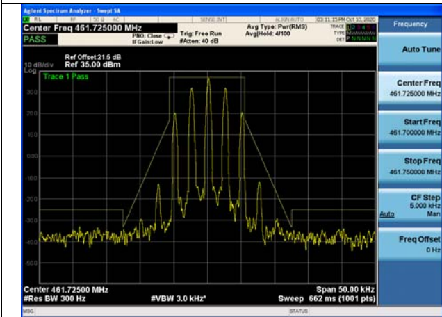
CH3
