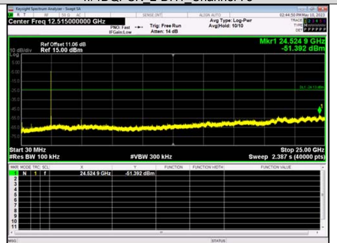
Spurious Emission \pi/4 DQPSK_2-DH1_Channel 78
