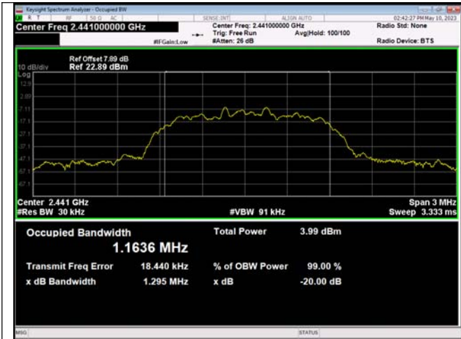
π/4DQPSK 2-DH1_Channel 39
