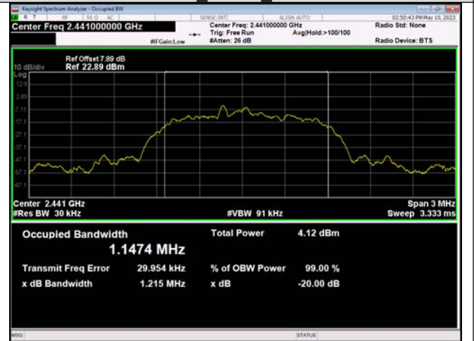
8DPSK 3-DH1_Channel 39
