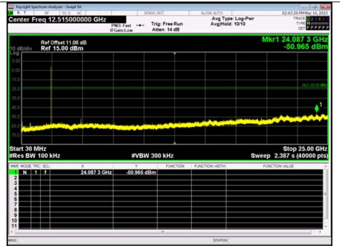
Spurious Emissions \pi/4 DQPSK_2-DH1_Channel 39
