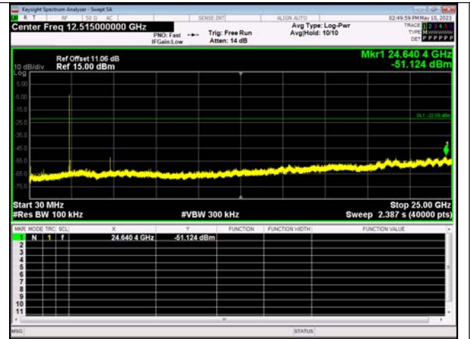
Spurious Emission 8DPSK_3-DH1_Channel 0
