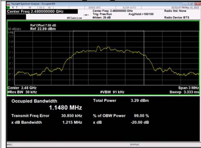
8DPSK 3-DH1_Channel 78
