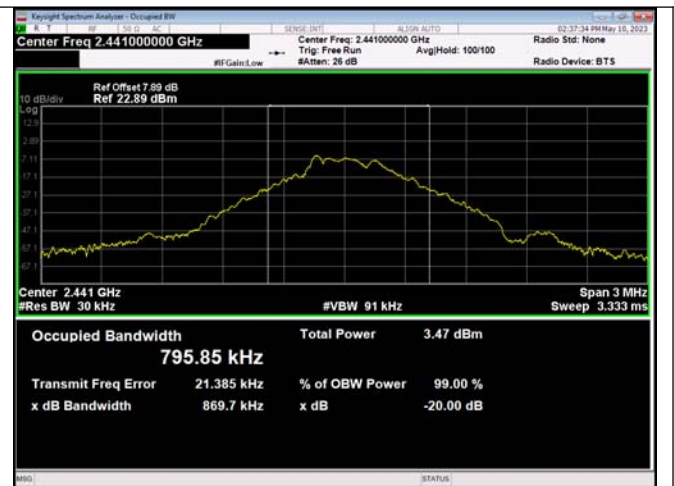
GFSK_DH1_Channel 39
