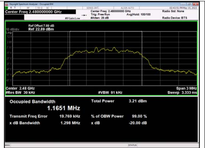
π/4DQPSK 2-DH1_Channel 78
