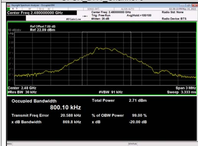
GFSK_DH1_Channel 78
