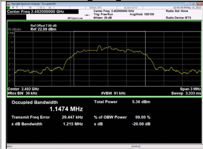
8DPSK 3-DH1_Channel 0
