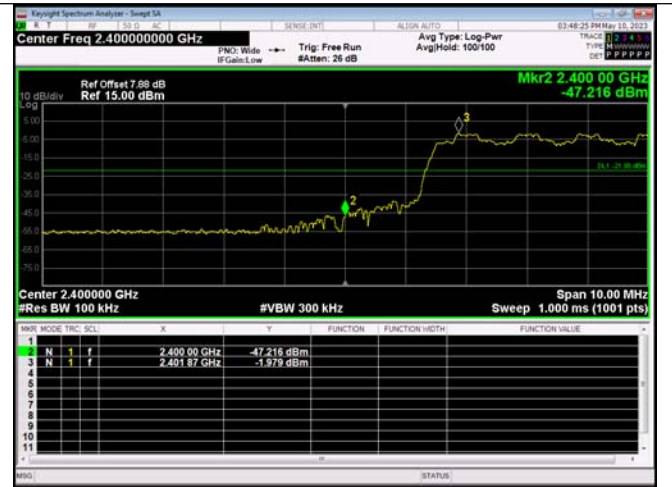
Out Of Band Emission(Left) \pi/4 DQPSK_2-DH1_Channel Hopping
