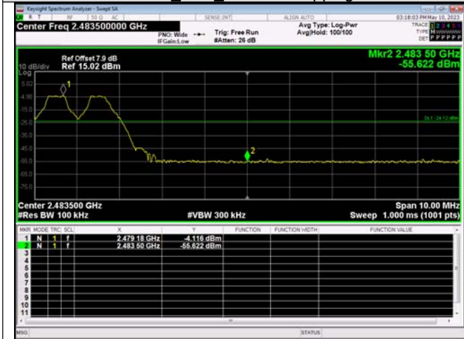
Out Of Band Emission(Right) GFSK_DH1_Channel Hopping
