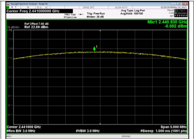
Peak Output Power 8DPSK_Channel 39
