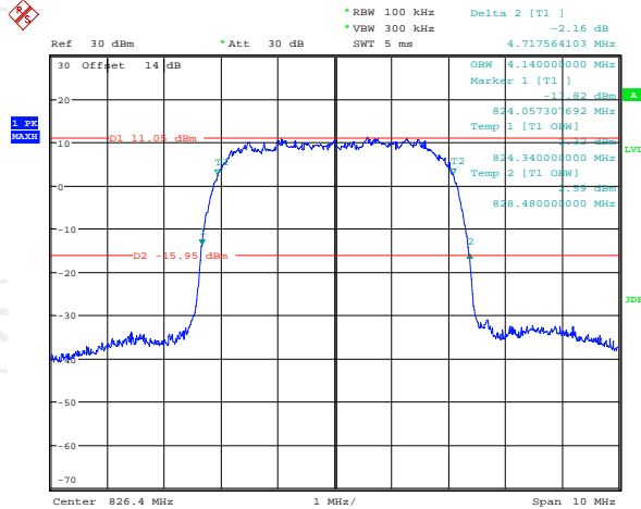
26dB&99% Occupied Bandwidth Plot on Channel 4132
