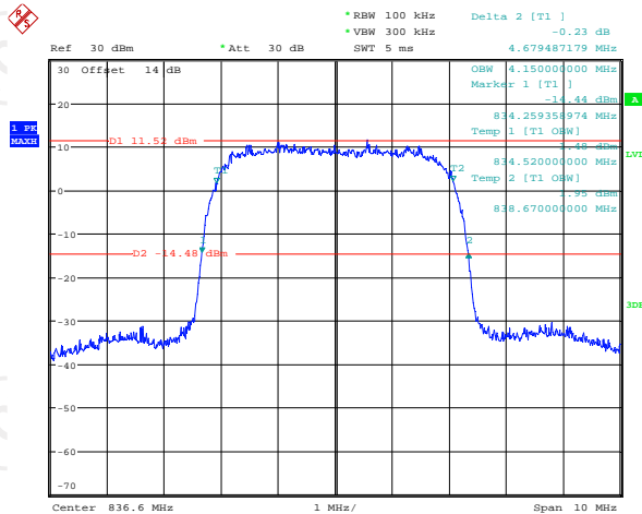
26dB&99% Occupied Bandwidth Plot on Channel 4183
