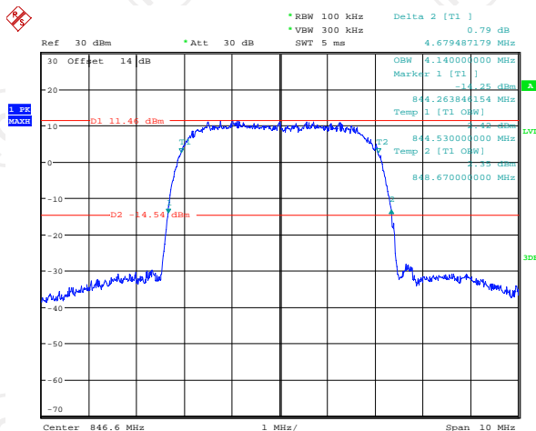
26dB&99% Occupied Bandwidth Plot on Channel 4233
