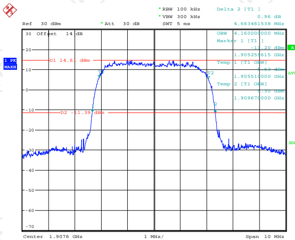
26dB&99% Occupied Bandwidth Plot on Channel 9538
