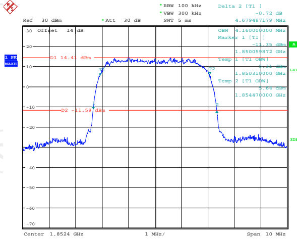
26dB&99% Occupied Bandwidth Plot on Channel 9262
