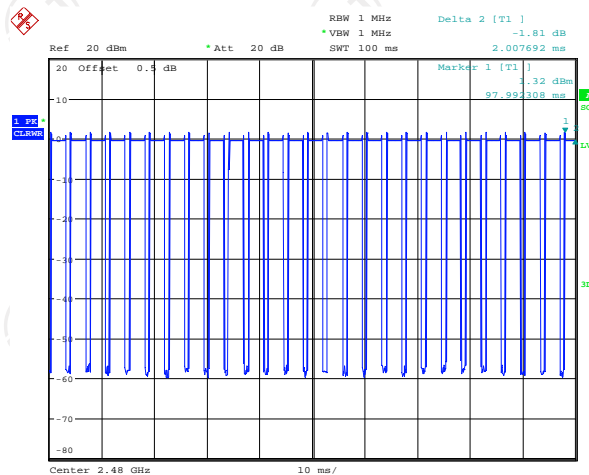
DH5 on time (Count Pulses) Plot on Channel 78
