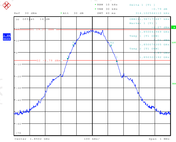
26dB&99% Occupied Bandwidth Plot on Channel 512
