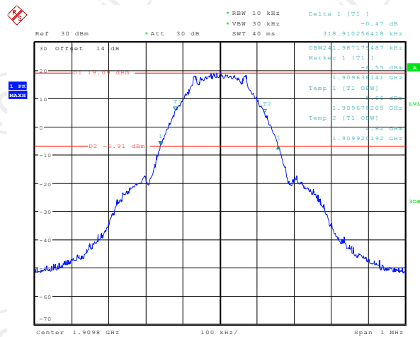
26dB&99% Occupied Bandwidth Plot on Channel 810
