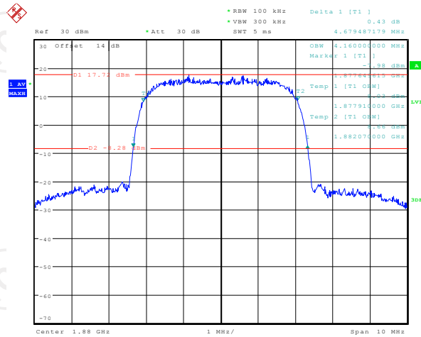
26dB&99% Occupied Bandwidth Plot on Channel 9400
