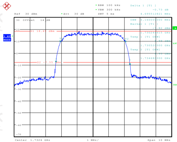
26dB&99% Occupied Bandwidth Plot on Channel 1413
