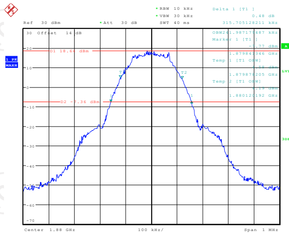
26dB&99% Occupied Bandwidth Plot on Channel 661
