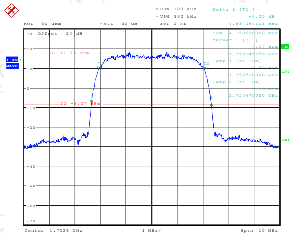
26dB&99% Occupied Bandwidth Plot on Channel 1513
