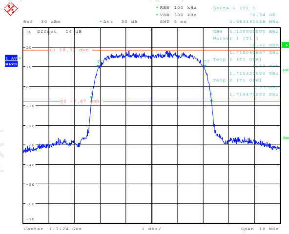
26dB&99% Occupied Bandwidth Plot on Channel 1312
