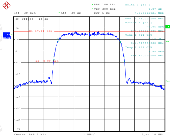
26dB&99% Occupied Bandwidth Plot on Channel 4233
