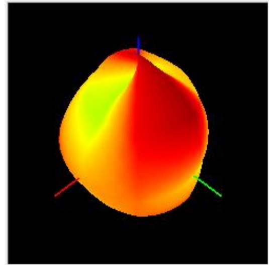
FDD- B66-TIS
