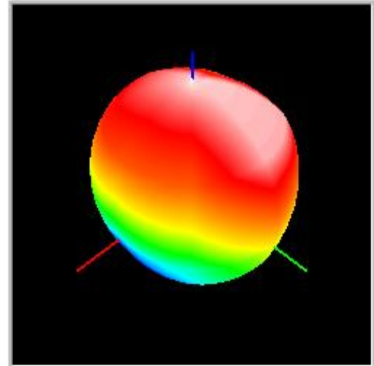
FDD- B17-TIS
