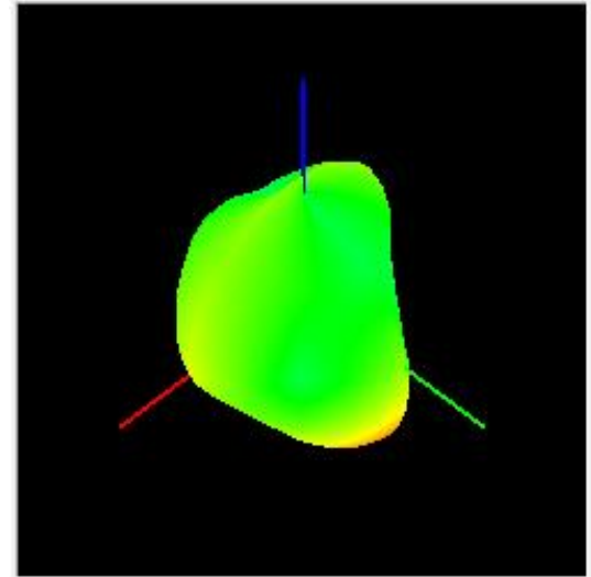
FDD-B5- TIS
