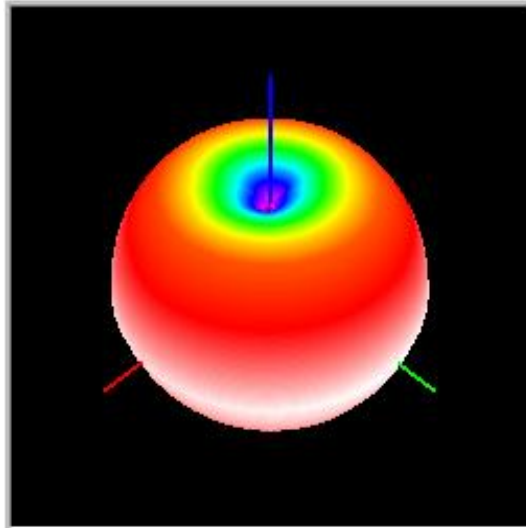
FDD- B12-TRP
