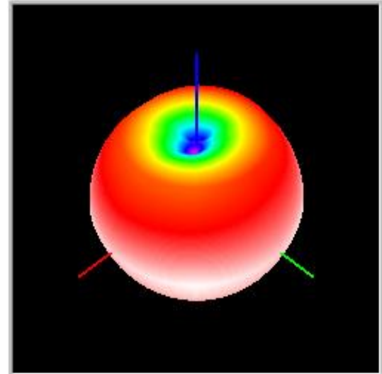
FDD- B12-TIS
