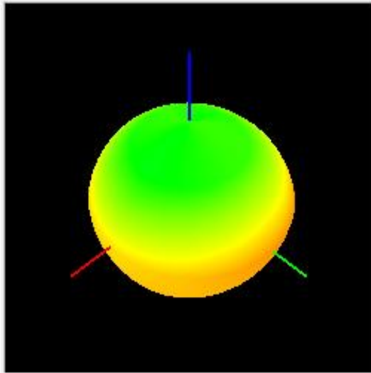
FDD- B71-TRP
