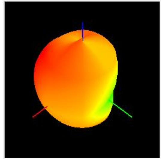
FDD-B4- TIS
