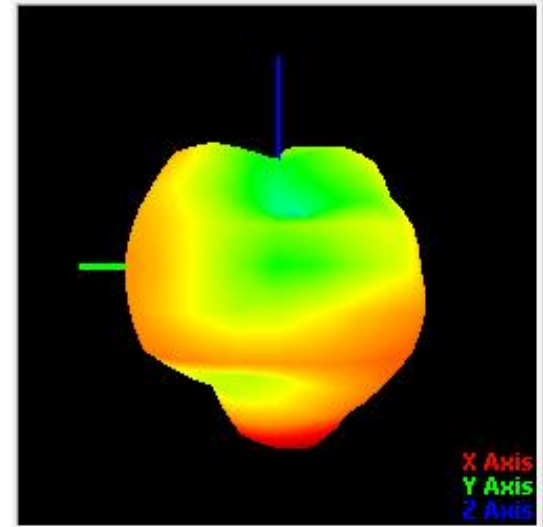
WIFI+BT- 2430MHZ
