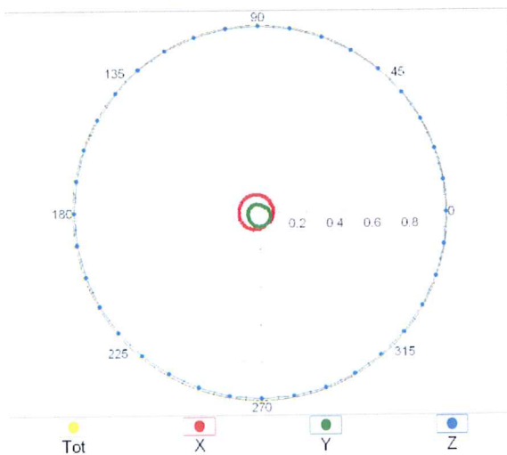
f=600 MHz,TEM,90°
