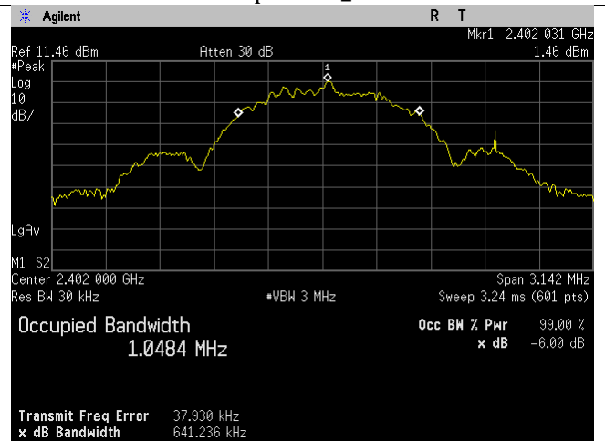
Low Ch_2402MHz_1MBit_Occupied Bandwidth_99percent_
