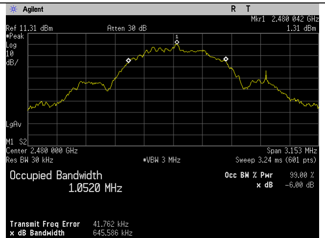
High Ch_2480MHz_1MBit_Occupied Bandwidth_99percent_
