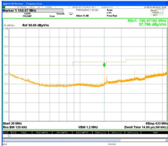
Plot # 5. Spurious emissions scan 30 MHz – 433.0 MHz.
