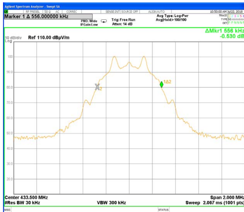
Plot # 13. Occupied bandwidth test result
