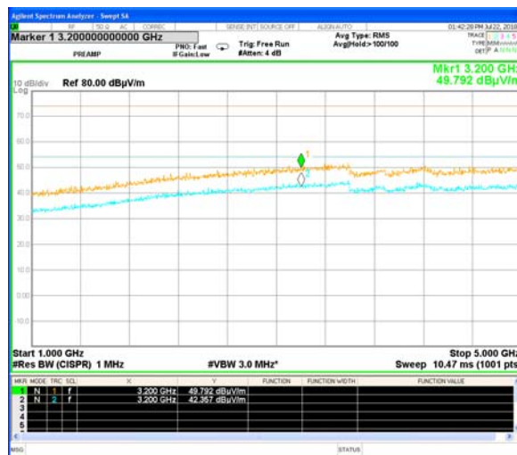
Plot # 7. Spurious emissions scan 1.0 – 5.0 GHz.
