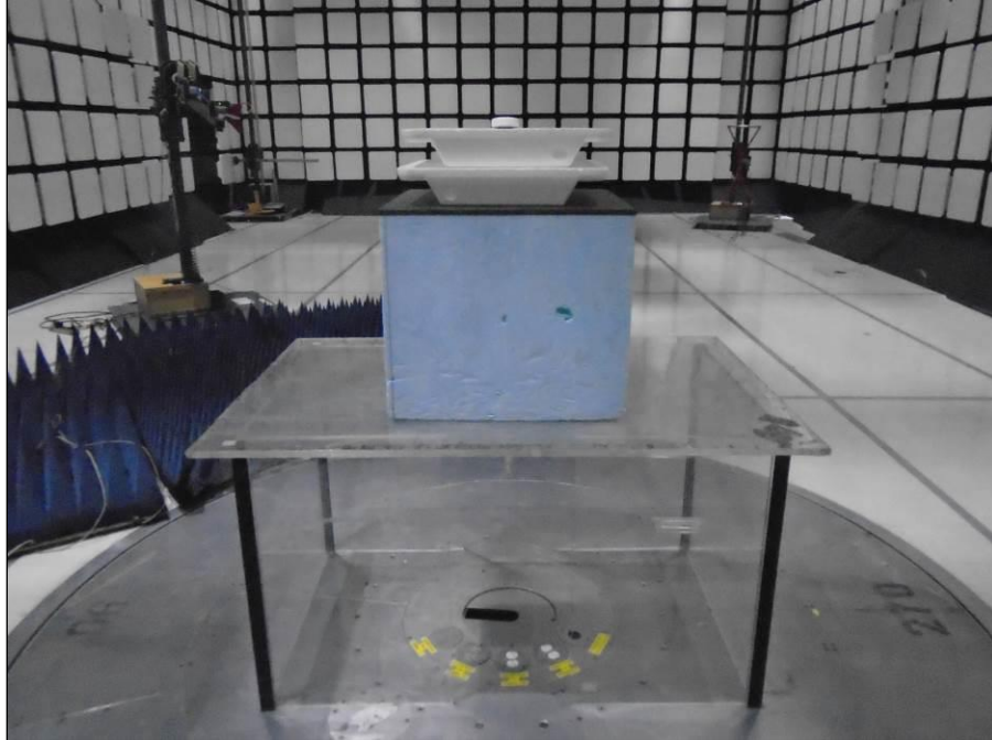
Photograph 3. Radiated Spurious Emissions, 1-10 GHz Setup Rear
