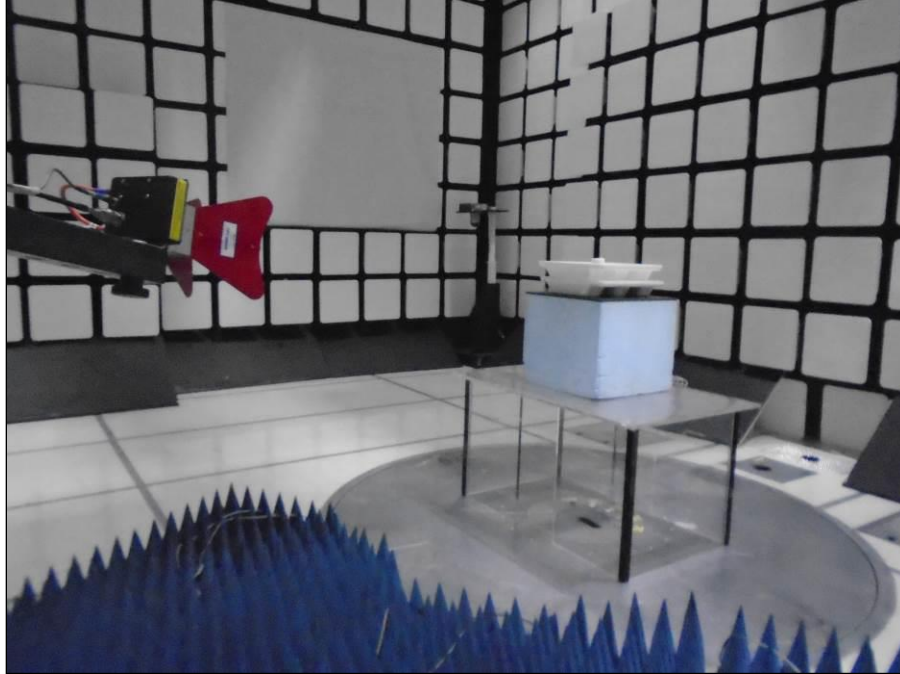
Photograph 1. Radiated Spurious Emissions, 1-10 GHz Antenna
