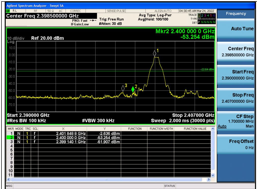
Test_Graph_EDR_ANT1_2402_1Mbps_Lower Band Edge Emissions
