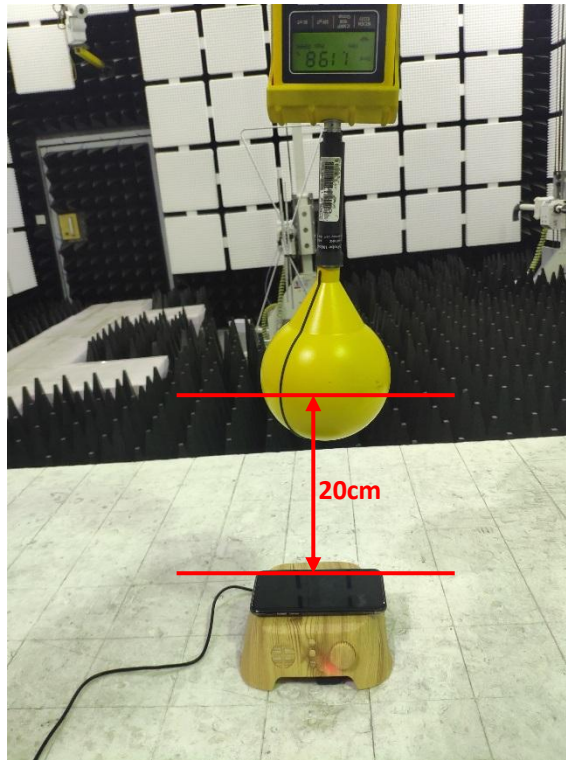
TestPosition E-Exposure photo from top surface (20cm)
