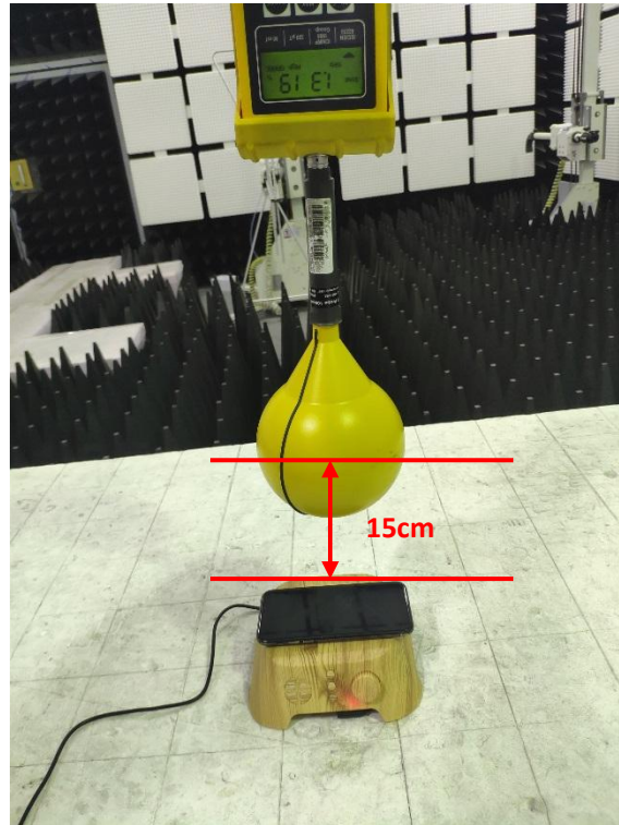
TestPosition E-Exposure photo from top surface (15cm)
