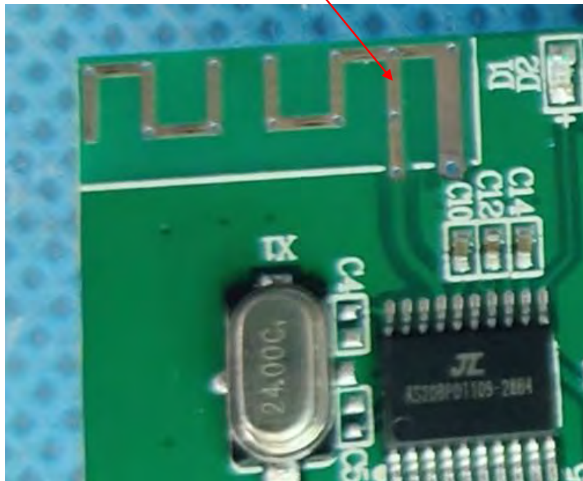
PCB Antenna
