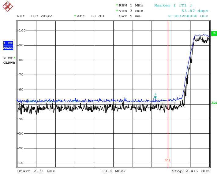
Radiated Restricted Band Edges plot – Peak Reading (802.11n_HT20 Ch.1)
