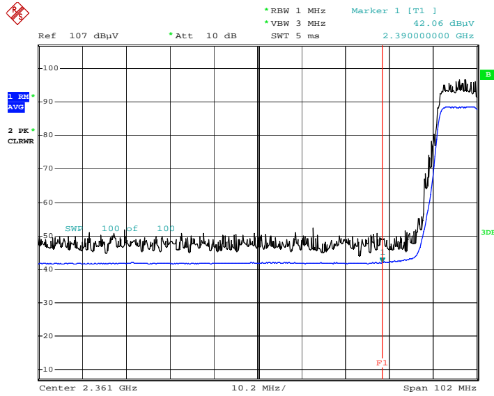
Radiated Restricted Band Edges plot – Average Reading (802.11n_HT20 Ch.1)
