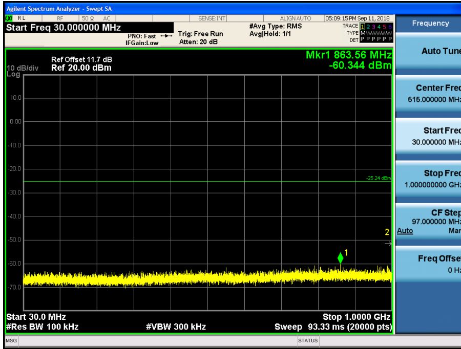
Conducted Spurious Emission (802.11g_Ch.11_12 Mbps)
