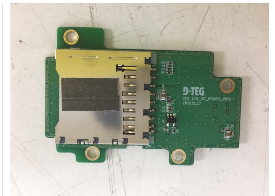
Bottom view of Sub3 PCB
