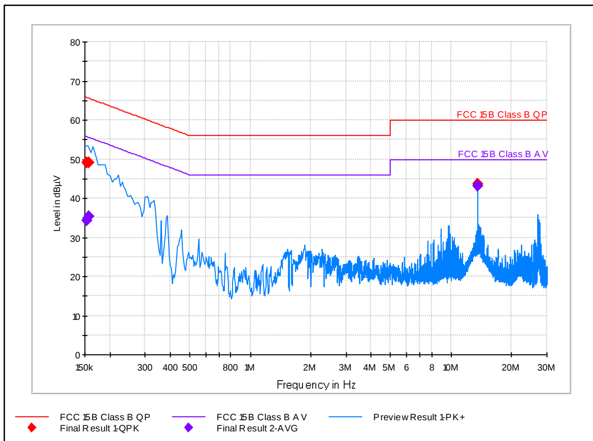
Figure 8. AC Conducted emission.
