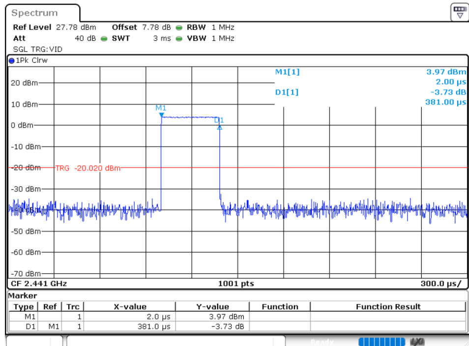
Dwell NVNT 1-DH1 2441MHz
