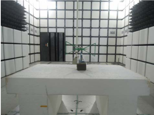
FCC_15_225_Radiated_Setup
