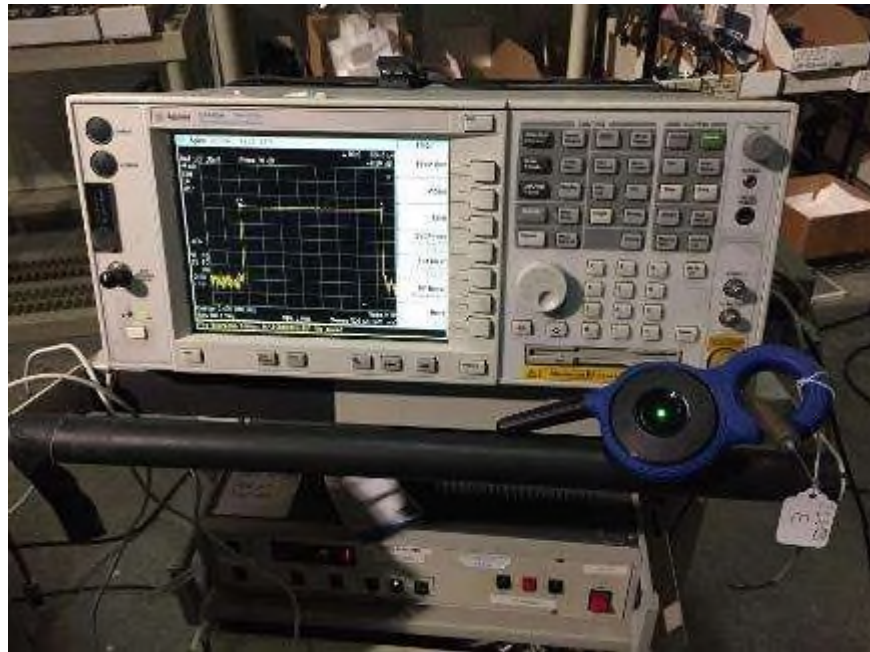
Timing Measurements
