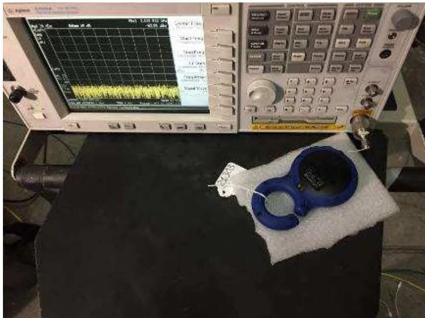
Conducted Antenna Port Measurements
