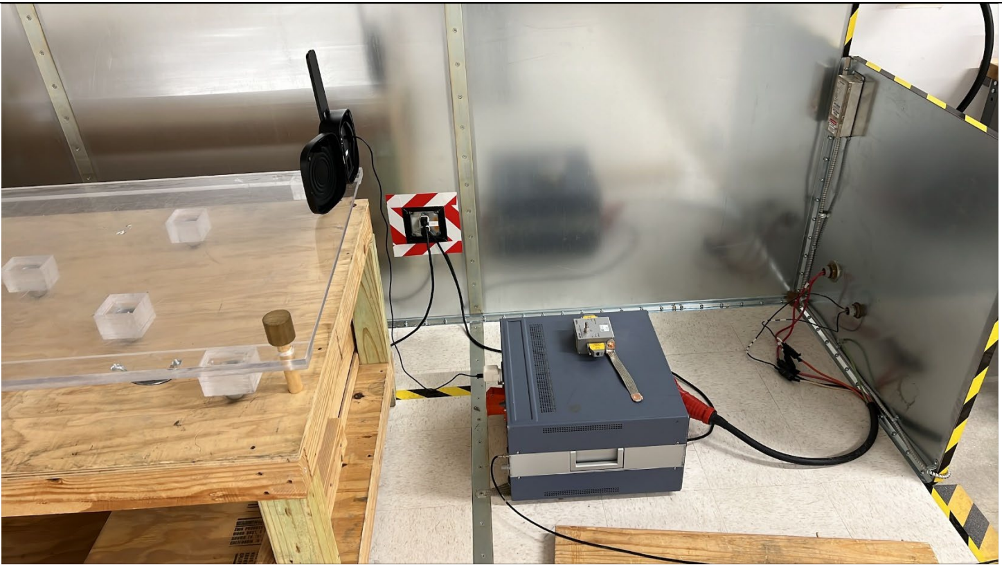
Conducted Emissions
