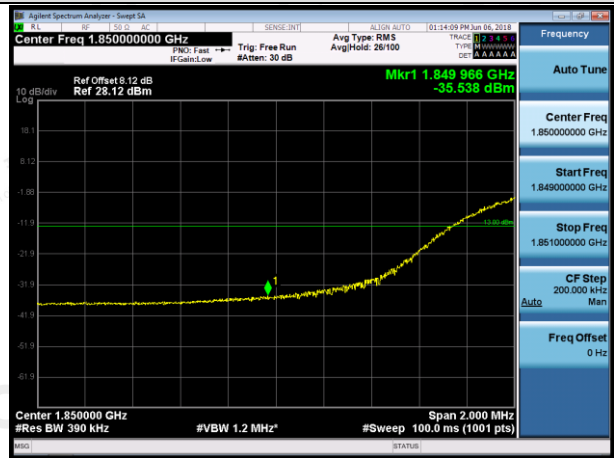
LCH_16QAM_100RB#0
