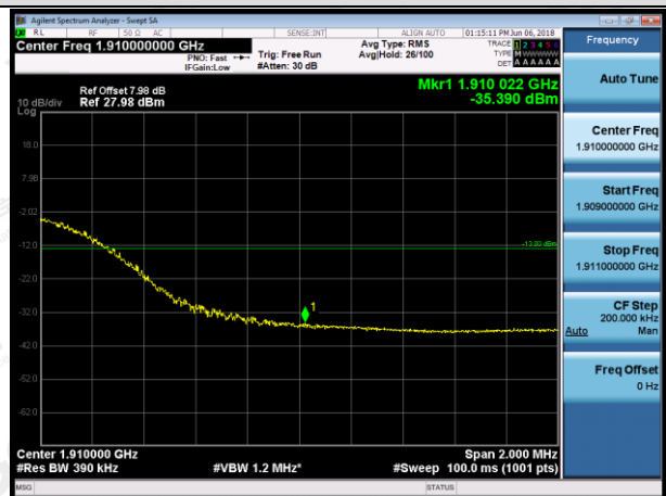
HCH_16QAM_100RB#0
