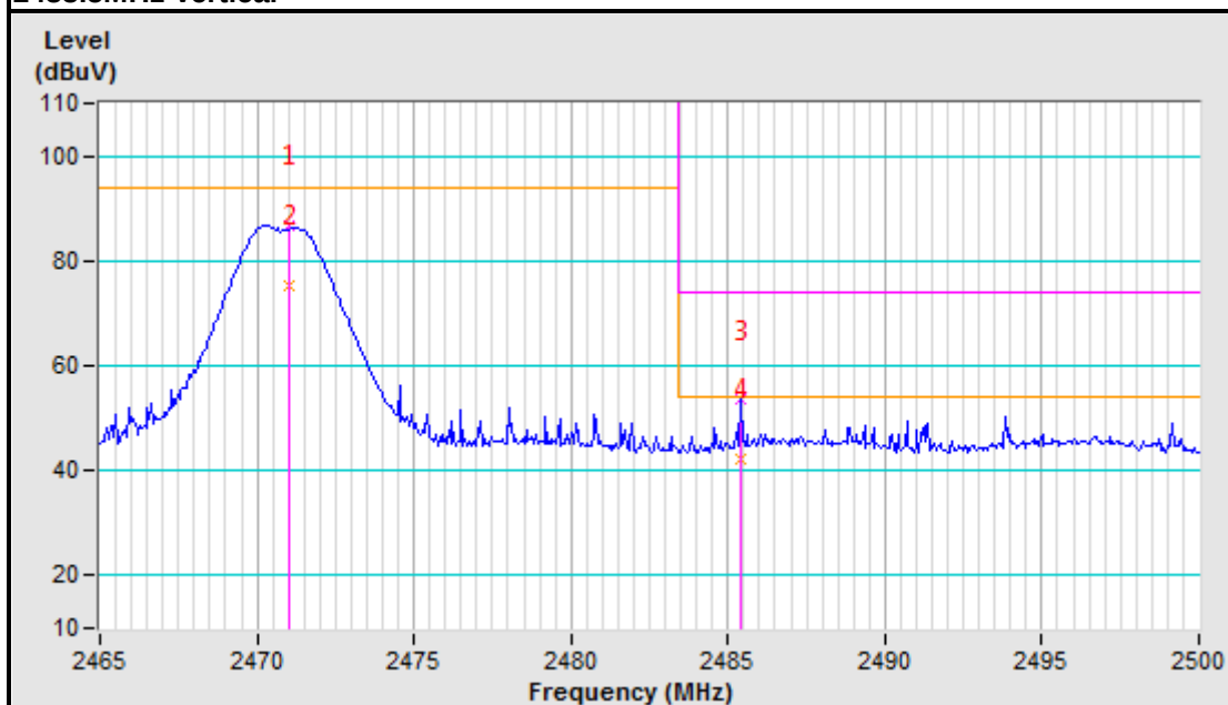
2483.5MHz Vertical
