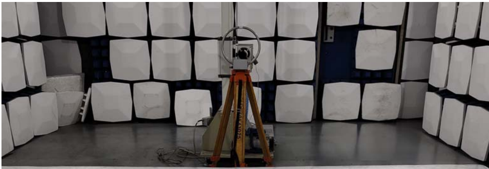
Radiated emission test view:
