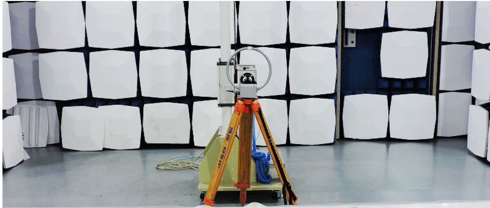
Radiated Emission Test Setup:
