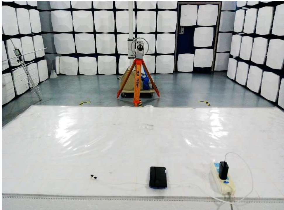
Radiated emission test view
